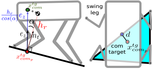
Fig. 6. Heuristic generation of the CoM target. (left) planning on inclined terrain, (right) the future support polygon is depicted in light blue while the projection x_{com_p}^{tg} of the com target on the polygon is a red dot.
