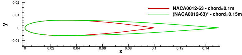
Figure 11: Profiles with different chord
