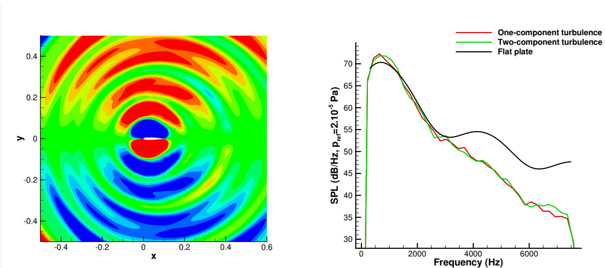
(a) Instantaneous pressure perturbation contour between \pm 4 Pa. (one-component turbulence).
