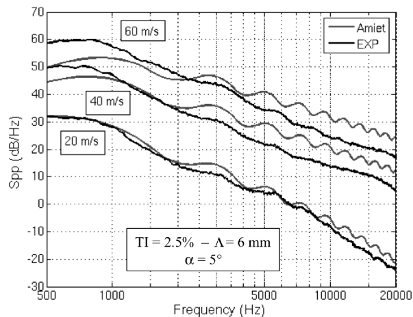
Figure 15. Predicted and measured PSD at 90^\circ .
