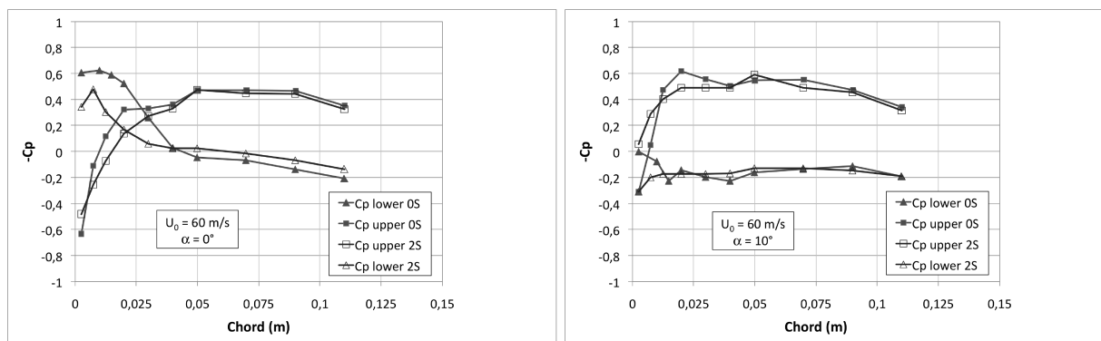
Figure 12. C_p distributions for baseline and 2S wings measured at \alpha = 0^\circ (left) and 10^\circ (right).
