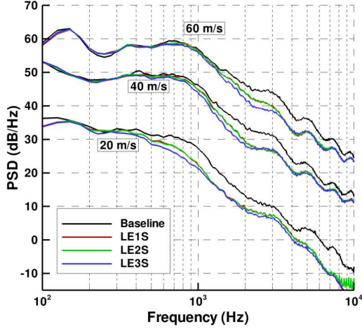
Figure 17. Baseline and serrated wing spectra at 90°.
