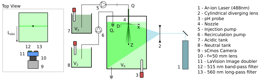
Fig. 10: Sketch of the setup designed for the turbulent jet experiment
