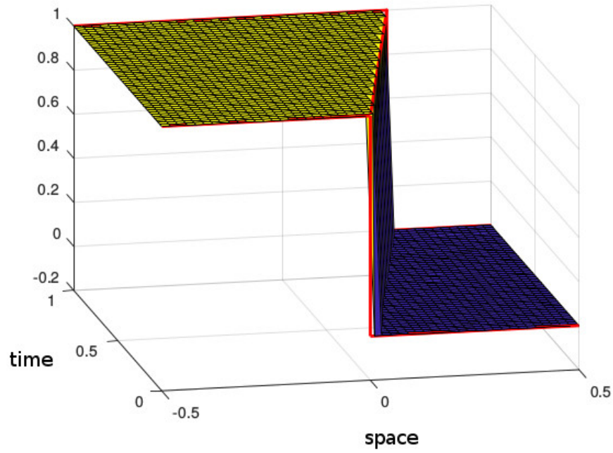
Figure 12: Graph of the solution (a function of time and space) recovered from approximate moments for the Burgers PDE: Discontinuous initial data. The shock propagates linearly with time.
