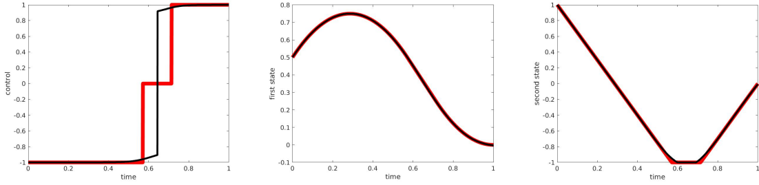
Figure 7: Minimum time double integrator with state constraint: control (left), first state (middle) and second state (right) trajectories (red) and their degree 8 semi-algebraic approximations (black) constructed from the pseudo-moments of the occupation measure.
