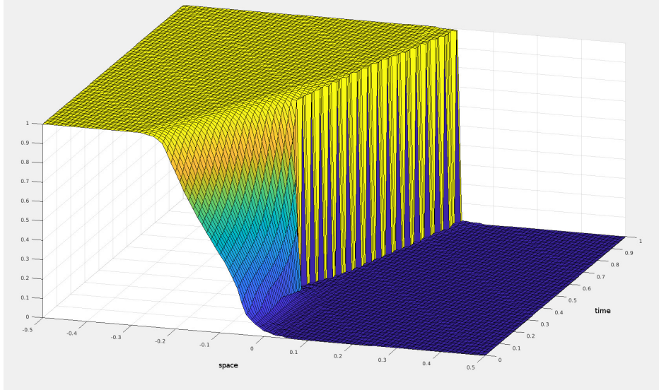
Figure 14: Graph of the solution (a function of time and space) recovered from approximate moments for the Burgers PDE: Initial function chosen such that the shock occurs at t = \frac{1}{2} .
