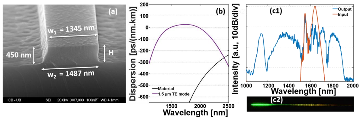
Figure 2. (a) Scanning Electron Microscope image of the cleaved strip waveguide (b) Dispersion properties for the fundamental TE 0,0 mode. (c1) Optical supercontinuum obtained at the output of the waveguide (solid blue line) compared to the input pulse spectrum (red solid line). (c2) Image of the emitted visible light from the waveguide (total length ~ 6.5 mm).
