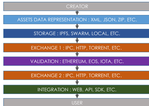
Fig. 2. Life cycle of a blockchain game asset
