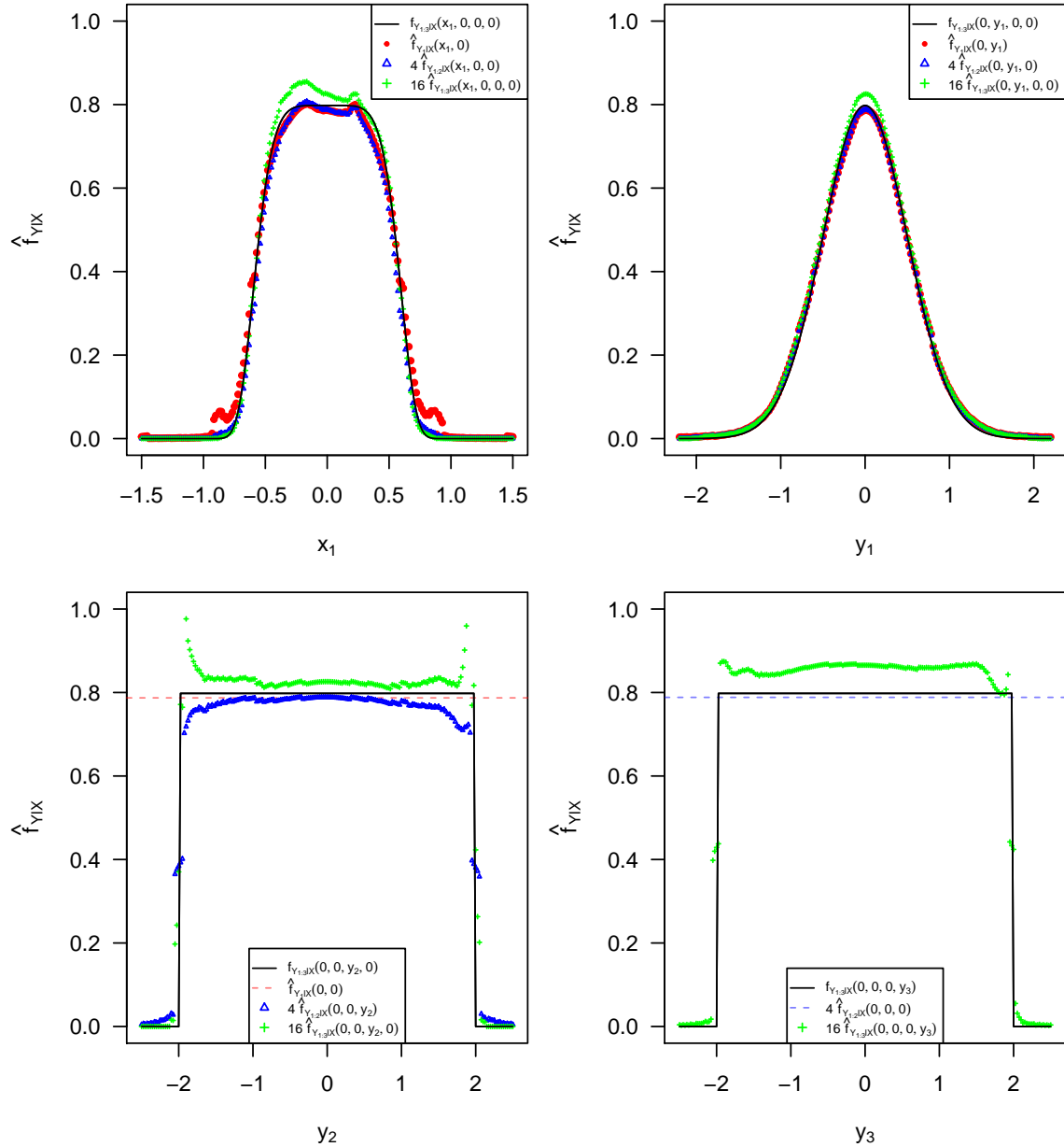
Figure 11: Estimation with sparsity in the response variables. The black straight line corresponds to the true renormalized conditional density varying along 4 directions: along x_1 top left, along y_1 top right, y_2 bottom left, along y_3 bottom right. In red: the pointwise estimates of f_{Y_1|X}(x, y_1) , in blue: those of f_{Y_{1:2}|X}(x, y_1, y_2) (multiplied by 4), in green: those of f_{Y_{1:3}|X}(x, y_1, y_2) (multiplied by 16).
