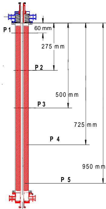
Th. couple locations in the adsorbent bed
