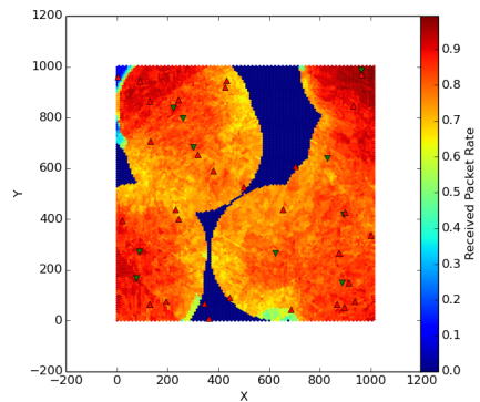
Figure 8. RPR with 30 noise nodes at h=60m
