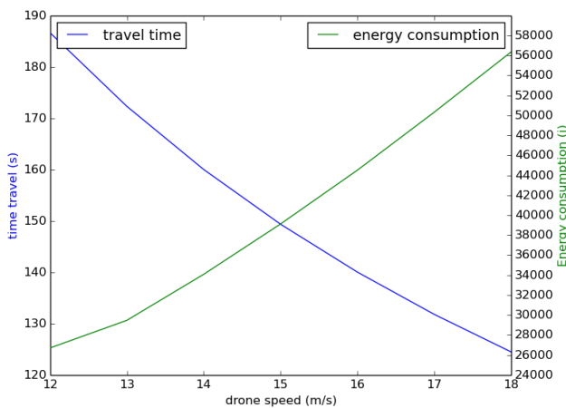
Figure 17. Energy consumption at different drone speeds
