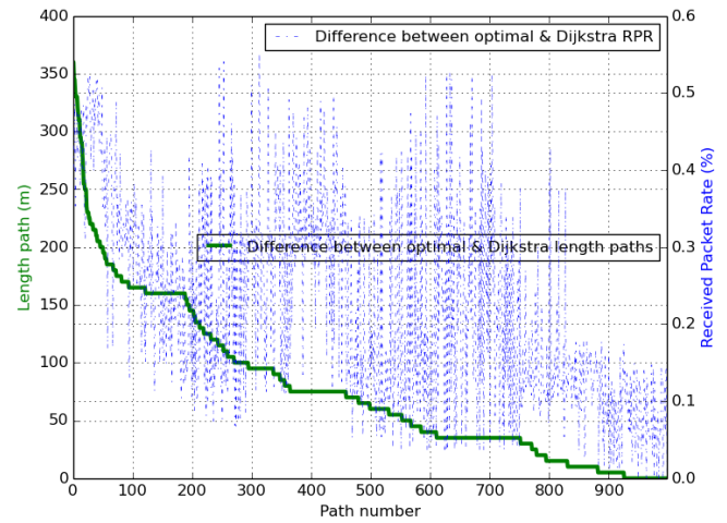
Figure 14. Difference between optimal and Dijkstra path length, nbr paths = 1000
