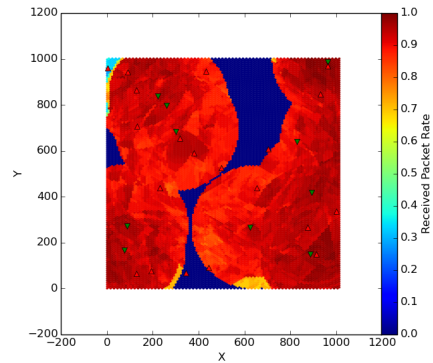
Figure 7. RPR with 20 noise nodes at h=60m
