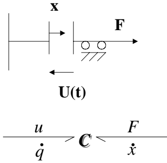
Figure 1. Variable Capacity
