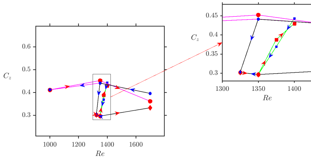
Figure 13: Hysteresis loop: C_z as a function of Re . The left hand side plot is the global view and the right hand-side plot shows a zoom into to loop. Three sequences of simulations are presented: the cases shown in Fig. 10 in green line with square markers and the cases shown in Fig. 11 in magenta lines with circular markers. In each sequence, the simulations in increasing branch are differentiated with the ones in decreasing branch by the arrows showing the direction of variation of Re . Additionally, the increasing branches are presented with slightly bigger red marker and red arrows, whereas the one in decreasing branch are with smaller blue marker and blue arrows.
