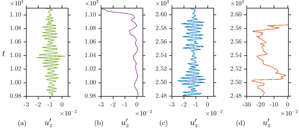
Figure 6: u'_z(0, 0, z, t) signal over time for Re = 1360 and \mathcal{A} = 0.2 recorded at z = 40d (a — ) and z = 80d (b — ). The time range of (a) and (b) are in LS, whereas the time range in (c) and (d) are in US2, recorded at z = 40d (c — ) and z = 80d (d — ). The time range in this figure are marked with the corresponding colour in Fig. 5(a).
