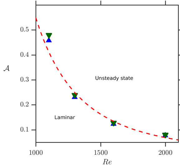
Figure 4: Critical amplitude, \mathcal{A} , of the vortex perturbation as a function of Re . The (green) triangles down indicate US and the (blue) triangles up LS. The (red) dashed line is power-law fit: \mathcal{A} \propto Re^{-3} .
