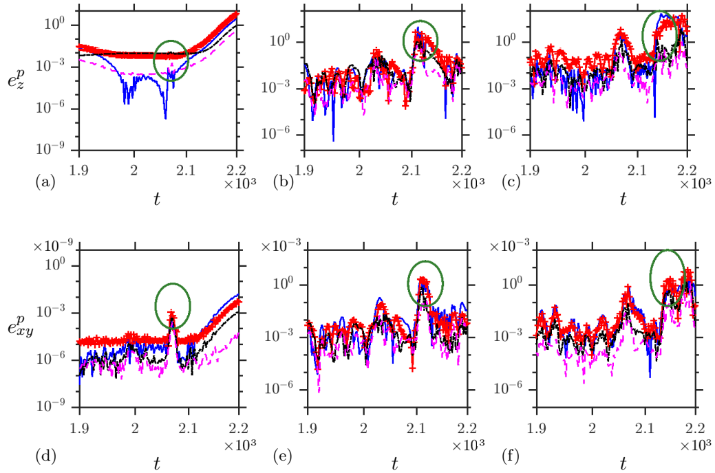
Figure 7: Time-evolution of the energy of the most relevant azimuthal modes at r = d/4 for Re = 1360 and \mathcal{A} = 0.2 . The colour code is: blue line for the mode 0, red (thick) line for the mode 1, black line for mode 2, and magenta line for mode 3. The three plots in upper row (a,b,c) show the energy of fluctuation pattern in streamwise direction, e_z , and the three plots in the lower row (d,e,f) show the energy of fluctuation pattern in spanwise direction. The three columns correspond to (a,d) z = 17d , (b,e) z = 47d and (c,f) z = 67d . The (green) circles indicate the peaks of energy.
