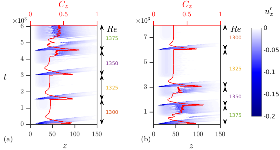
Figure 10: Hysteresis loop of transitional flows for \mathcal{A} = 0.2 . (a) Space-time diagrams of the increasing Re , (cases 3a, 4a, 6a and 7a) and (b) the decreasing Re , (cases 7b, 6b, 4b and 3b) branches. The diagrams also indicate the value of C_z as a (red) continuous line labeled on the top and the corresponding values of Re on the right.
