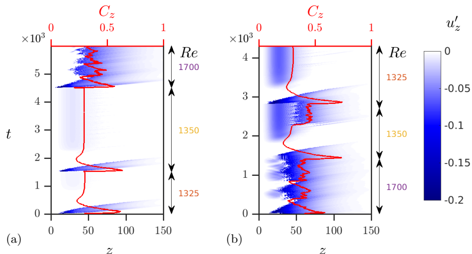
Figure 12: Hysteresis loop of transitional flows for \mathcal{A} = 0.5 . (a) Space-time diagrams of the increasing Re (cases L1d, L2d, L3dbis) and (b) the decreasing Re (cases 3a, 4a and 10a) branches. The diagrams also indicate the value of C_z as a (red) continuous line and the corresponding value of Re on the right.
