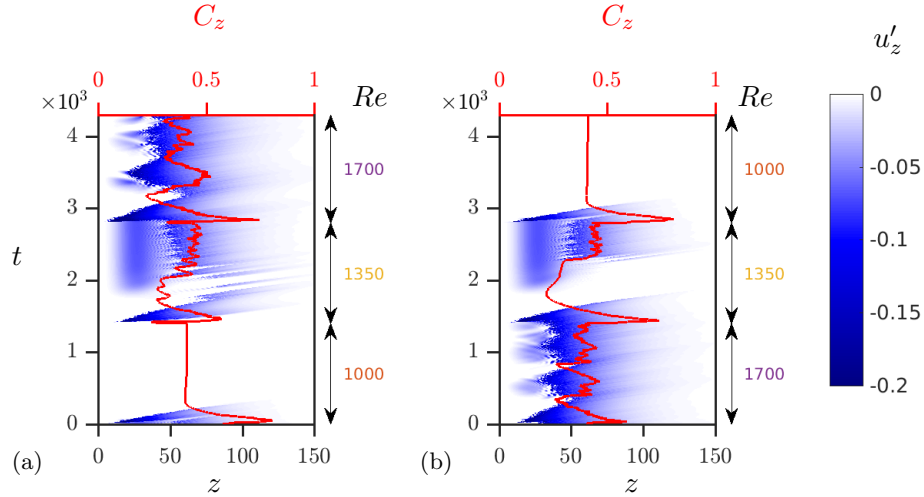
Figure 11: Hysteresis loop of transitional flows for \mathcal{A} = 0.2 . (a) Space-time diagrams of the increasing Re (cases L1d, L2d and L3d) and (b) the decreasing Re (cases L3d, L2i, L1i) branches. The diagrams also indicate the value of C_z as a (red) continuous line labeled on the top and the corresponding values of Re on the right.
