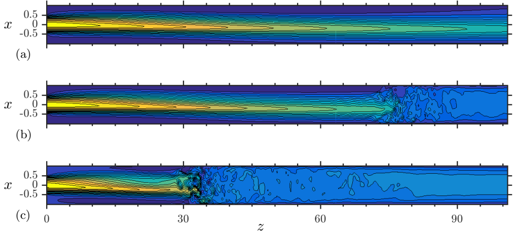
Figure 3: Contour plot of instantaneous streamwise velocity at Re = 2000 , y = 0 and zoomed into the range of 0 < z < 100d . (a) LS at \mathcal{A} = 0.09 , t = 750 , (b) US2 at \mathcal{A} = 0.09 , t = 1250 and (c) US1 at \mathcal{A} = 0.2 , t = 1000 .
