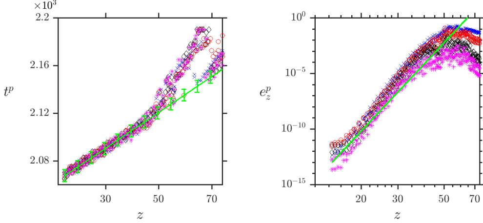
Figure 9: Tracking position of the energy peak for Re = 1360 and \mathcal{A} = 0.2 . (a) Time and axial position with the scaling represented as a (green) line: t^p = z/V_0 + c_1 , c_1 is a constant and the different colours represented different radial position. (b) Energy peak amplitude, e_z^p , versus axial position, z , for the first four modes: mode 0 ( \times ), mode 1 ( \circ ), mode 2 ( \diamond ), mode 3 ( * ), with the scaling in (green) line e_z^p = c_2 z^{20} where c_2 is a constant.
