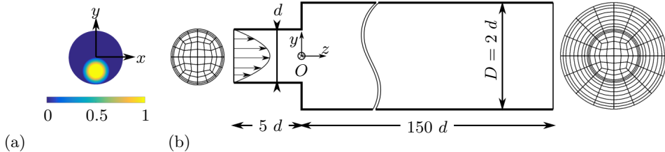
Figure 1: (a) Axial vorticity of the vortex perturbation ( R_\Omega = d/4 , (x_\Omega, y_\Omega) = (0, -d/4) and \mathcal{A} = 1 ) and (b) Sketch of fluid domain with 2 cross-sections inlet and outlet mesh.
