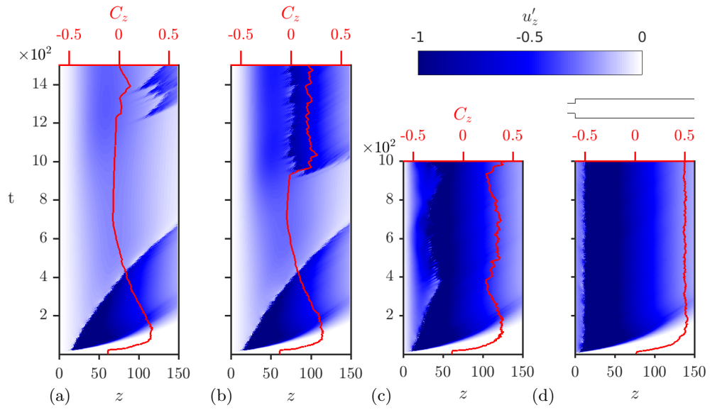
Figure 2: Space-time diagrams of the centreline perturbed streamwise velocity, u'_z , and drag coefficient, C_z , as a (red) line, indicated on the top, for Re = 2000 at (a) \mathcal{A} = 0.0782 , (b) \mathcal{A} = 0.09 , (c) \mathcal{A} = 0.2 and (d) \mathcal{A} = 0.5 . All the diagrams use the same colour code shown on the top right corner, such that light colour corresponds to laminar flow. The whole pipe section downstream the expansion, up to z = 150d , is also sketched in the top right corner below the colour bar.
