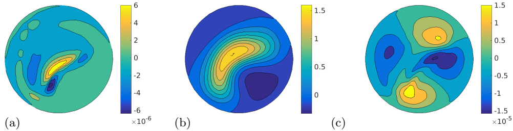
Figure 8: Contour plot in the cross-sectional plane at z = 17d for Re = 1360 and \mathcal{A} = 0.2 . (a) u_z^p(z = 17d) = u_z(z = 17d, t_p = 2080) - u_z(z = 17d, t = 2070) , (b) mean flow: \bar{u}_z(x, y, z = 17d) and (c) regular unsteady pattern that remains bounded over time: u'_z(x, y, z = 17d, t = 2070)
