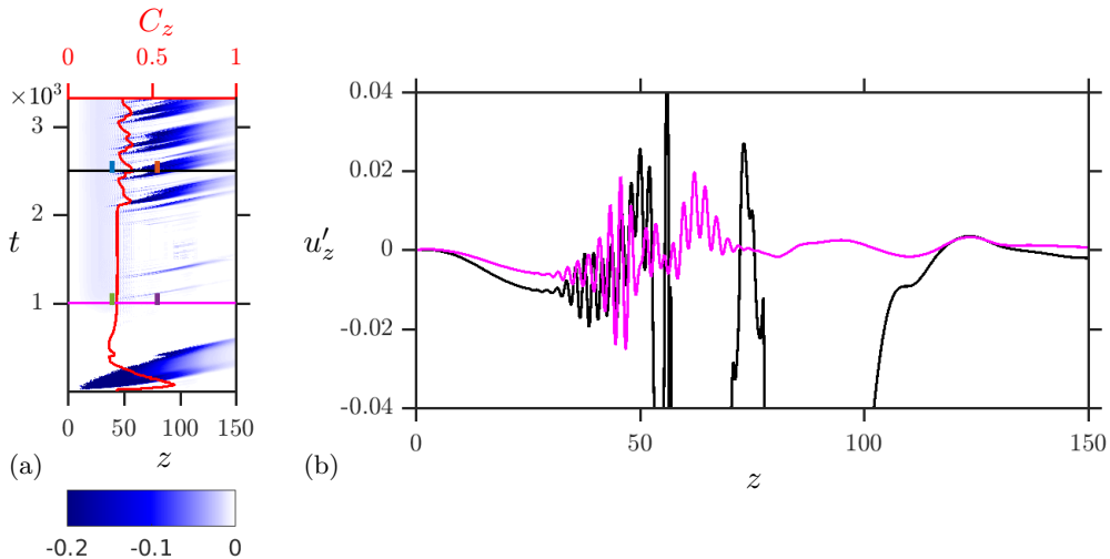
Figure 5: (a) Space-time diagram for Re = 1360 and \mathcal{A} = 0.2 , corresponding to case 5a. (b) u'_z(0, 0, z, t) profiles along the centreline at t = 1000 (LS —) and t = 2500 (US2 —).
