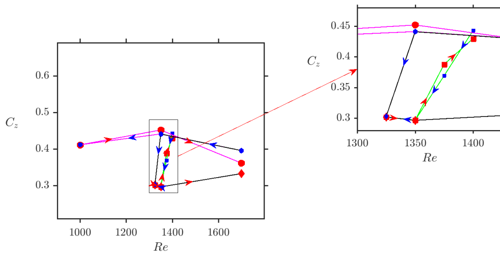
Figure 13: Hysteresis loop: C_z as a function of Re . The left hand side plot is the global view and the right hand-side plot shows a zoom into to loop. Three sequences of simulations are presented: the cases shown in Fig. 10 in green line with square markers and the cases shown in Fig. 11 in magenta lines with circular markers. In each sequence, the simulations in increasing branch are differentiated with the ones in decreasing branch by the arrows showing the direction of variation of Re . Additionally, the increasing branches are presented with slightly bigger red marker and red arrows, whereas the one in decreasing branch are with smaller blue marker and blue arrows.
