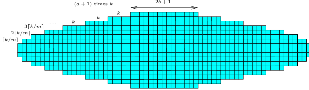
Figure 1: S_m^k(a, b) with m = 5 , k = 5 , a = 2 and b = 7 .
