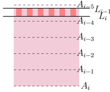
FIGURE 9. All vertices that need to be connected by an edge must be in the part of \mathcal{Q} between L_{i-1} and A_i .
