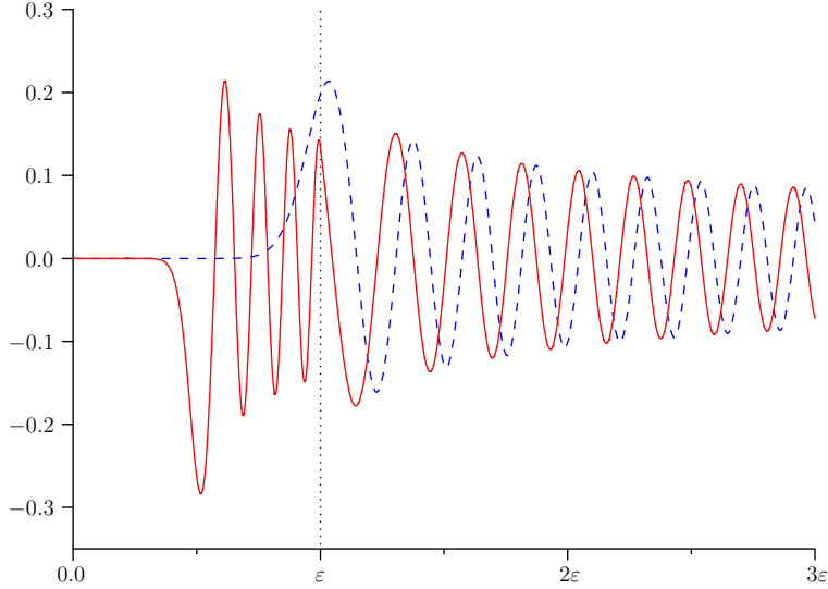
FIGURE 4.2. Last quasi-resonant solution for \lambda = 2 and n = 30 .
