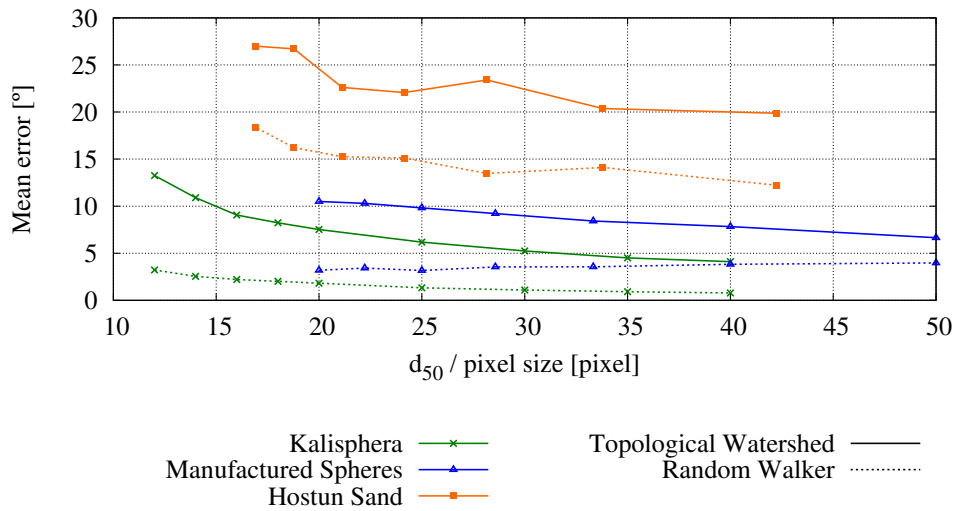
Figure 16: Results of the contact orientation study on the high resolution tomographic images of the manufactured spheres (blue lines) and Hostun Sand (orange lines) for the topological watershed (solid lines) and the random walker (dotted lines). The results of the study on synthetic images of spheres in contact are added for comparison (green lines).
