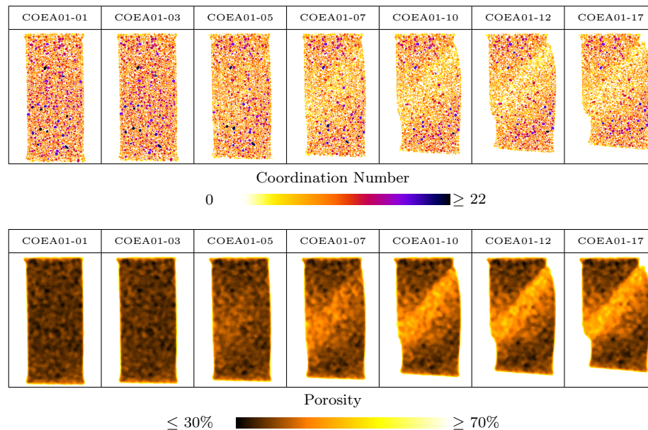
Figure 7: Slices from some selected states in the test COEA01. In the top row, each grain is coloured by its coordination number; in the bottom row field of local porosity measurements
