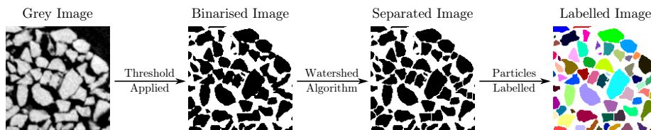
Figure 4: Very simplified illustration of the grain-identification procedure used
