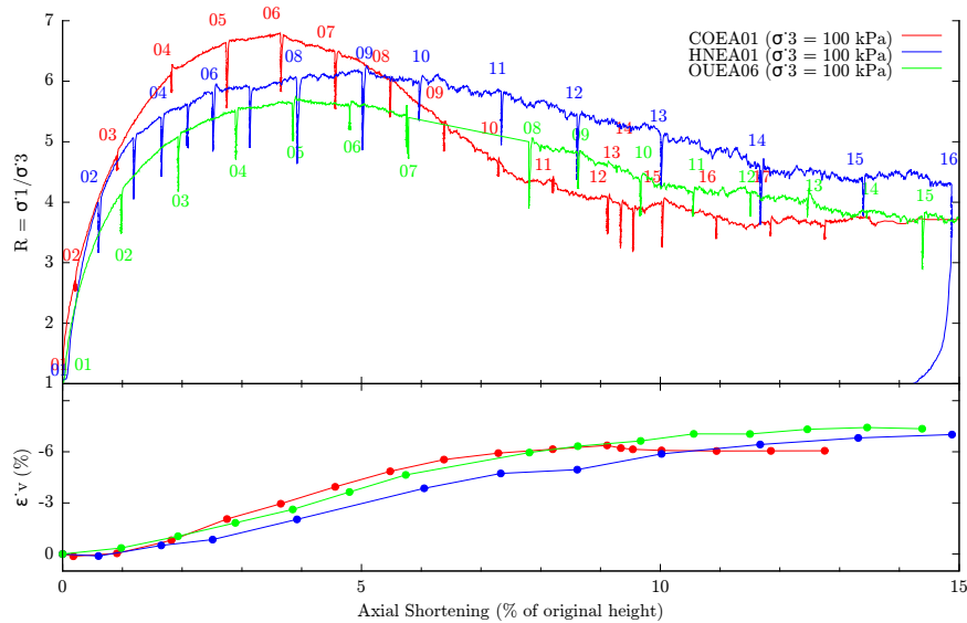
Figure 5: Triaxial test responses for three tests on Caicos Ooids (COEA01), Ottawa sand (OUEA06) and Hostun sand (HNEA01), performed at a cell pressure of \sigma_3 = 100 kPa. The volumetric strain ( \epsilon_v ) response of each material is dilatant.
