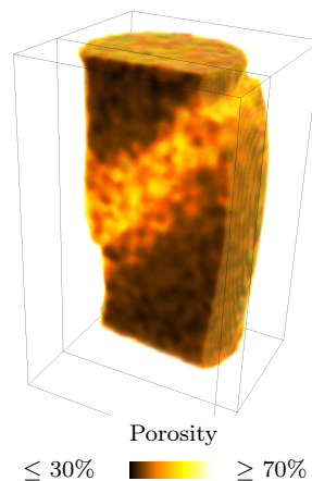
Figure 6: 3D rendering of the porosity field of state COEA01-17
