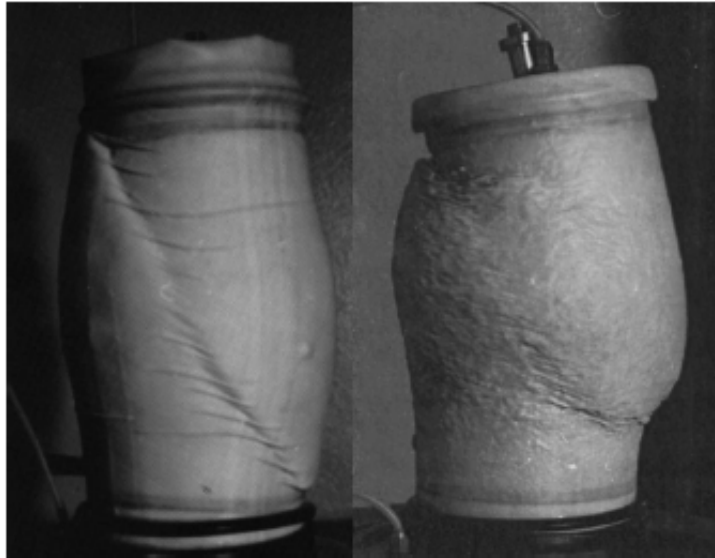
Figure 1: Shear bands observed in triaxial specimens on fine and coarse sand, left and right respectively
