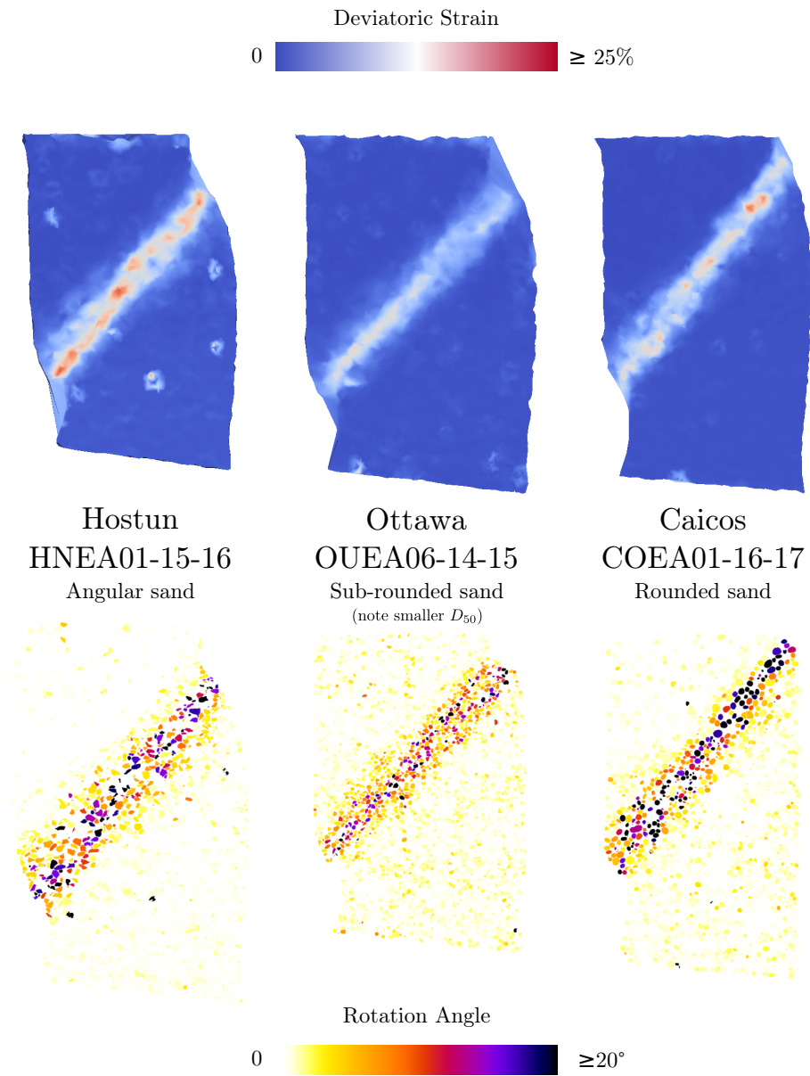
Figure 9: Deviatoric strain and grain rotations in the final increments of COEA01, OUEA06, HNEA01, adapted from [29]
