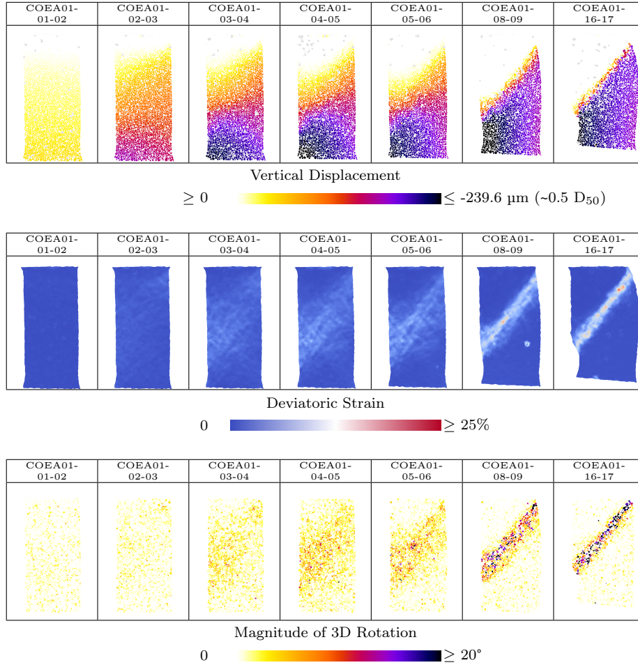
Figure 8: Slices from some selected increments in the test COEA01. In top and bottom rows, each grain is coloured by a scalar quantity (vertical displacement (negative = upwards) or magnitude of 3D rotation over an increment) with untracked grains are shown in light grey. In the middle row a field of deviatoric strain is shown
