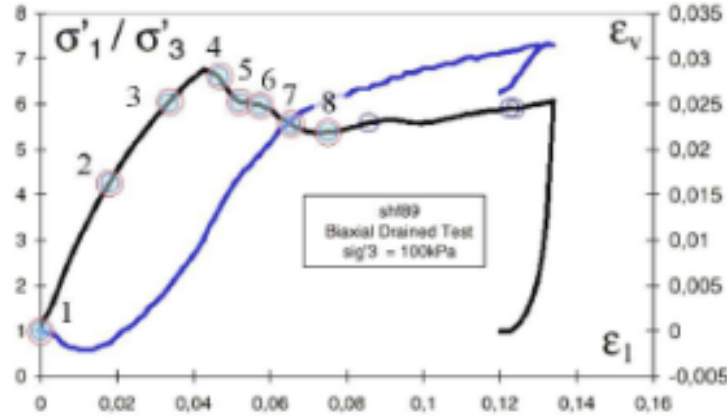
Figure 3: Stress-strain response of specimen shf89 . In black the stress ratio ( \sigma_1/\sigma_3 ) against axial strain ( \epsilon_1 ). In blue the volumetric strain response ( \epsilon_v ) against axial strain
