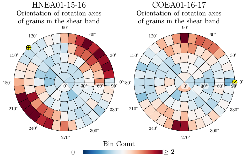
Figure 10: Comparison of the rotation axes for the grains in the shear band in specimens HNEA01 and COEA01. The yellow dot indicates the orientation of the direction of maximum slope in the shear band
