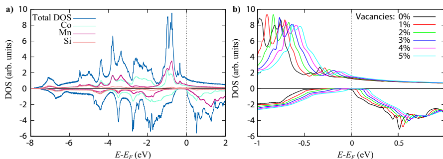
Figure 1. Spin-resolved DOS of \text{Co}_2\text{MnSi} , a) for the perfect \text{L2}_1 phase (with partial contributions of Co, Mn and Si atoms), b) near the Fermi level E_F , as a function of the percentage of vacancies x . Upper and lower panels respectively correspond to majority and minority spin electrons.
