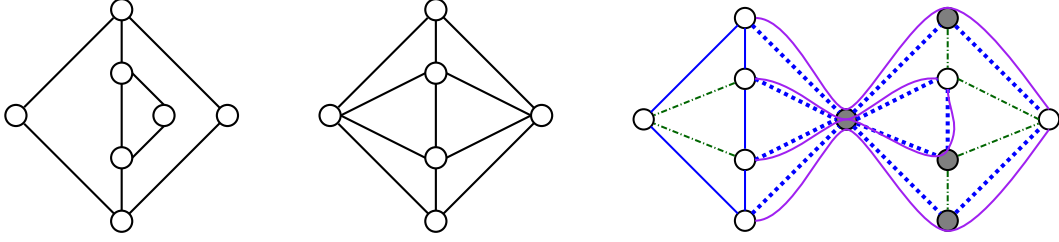
Fig. 3 Left: Motif A . Center: Motif B . Observe that A \not\mapsto B . Right: Motif A is embedded into two consecutive Motifs B : solid lines are virtual links mapped on single substrate links, solid curves are virtual links mapped on multiple substrate links, dotted lines are substrate links implementing a multi-hop virtual link, and dashed lines are substrate unused links. Grayed nodes are relay-only nodes. Observe that the central node has a relaying load of 4\epsilon .
