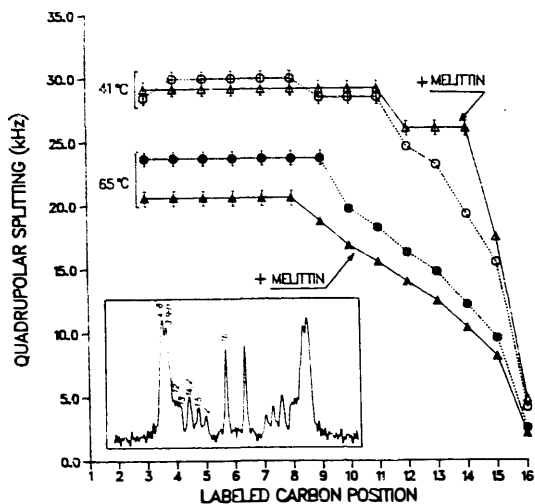
Fig. 3. Quadrupolar splittings from de-Paked spectra ( see insert ) of [sn-2- 2 H 31 ]DPPC in the presence ( Ri = 20) and in the absence of melittin at 41°C and 65°C, as a function of the labeled carbon position along the sn-2-acyl chain. Prime numbers in the de-Paked spectrum ( insert ) represent the assignment of labeled positions.
