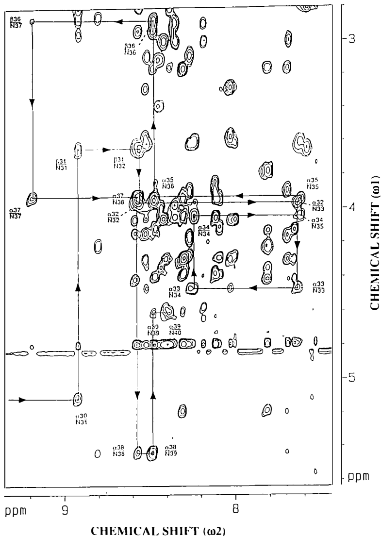
Fig. 3. Part of a 500 MHz NOESY (150 ms) spectrum of recombinant defensin A in ^2\text{H}_2\text{O} (pH 4.9, 8.9 mM, 294 K). The sequential pathway ( i, i + 1 ), mainly involving d_{\alpha\text{N}} connectivities (see text), is displayed from Cys 30 to Asn 40 .
