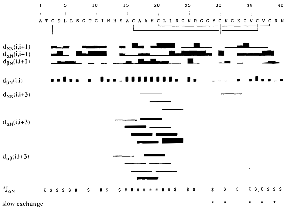
Fig. 4. Summary of some short and medium-range NOE connectivities observed in a 500 MHz NOESY (150 ms) spectrum of recombinant defensin A (pH 4.9, 8.9 mM, 294 K). The sequence is displayed with the one-letter code and the 3 disulfide bridges are enhanced by solid lines. The intensity of NOEs is classified as strong, medium and weak by the height of lines. Amide protons in slow exchange with ^2\text{H}_2\text{O} at 283 and 294 K are indicated by a star. ^3J_{\text{NH}-\alpha\text{H}} values measured from DQF-COSY experiments at 313 K are classified as large (£ \geq 9 Hz), medium ( 7 \text{ Hz} \leq S < 9 \text{ Hz} ) and small ( \# < 7 \text{ Hz} ).
