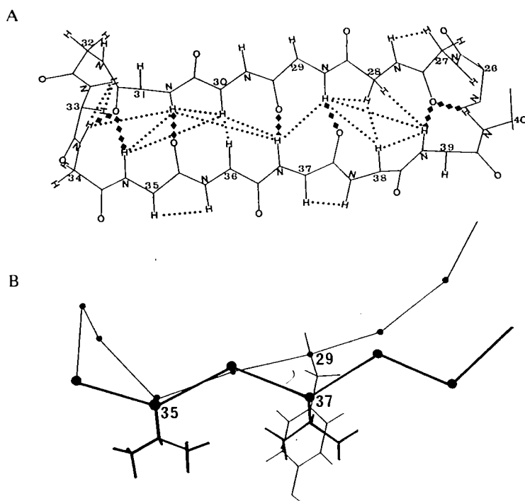
Fig. 7. The \beta -sheet structure (model A 4 ; see text) of the C-terminal fragment of recombinant defensin A. In (A) the backbone is displayed from Arg 26 to Asn 40 and C \alpha atoms are numbered. Hydrogen bonds are represented by filled diamonds (◆) and only a selection of typical (i,i+1) and interstrand NOEs is shown by dotted lines. (B) represents a profile view of (A) with respect to a horizontal axis. Among the backbone, only C \alpha atoms (●) are shown in (B) and bold lines enhance the foreground strand. Side chains of Tyr 29 , Val 35 and Val 37 are also displayed.
