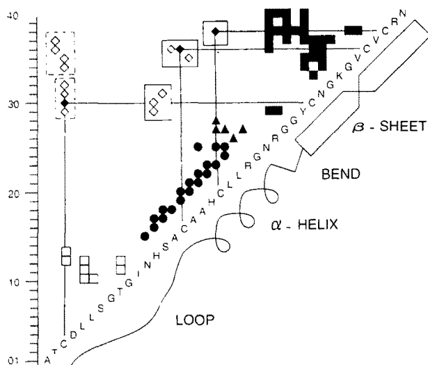
Fig. 6. Summary of medium and long-range connectivities ( i, j \geq i + 3 ) observed in NOESY maps (500 MHz, 150 ms) of recombinant defensin A in 1 H 2 O or 2 H 2 O ( p^1H = p^2H 4.9, 294 K). The sequence is displayed on the diagonal (one-letter code) with elements of secondary structure in which residues are involved. Symbols may represent more than one NOE between two residues of the diagonal. (◊), loop; (●), \alpha -helix; (▲), bend; (■), \beta -sheet. Off-diagonal diamonds placed in dashed boxes and solid boxes connect the two strands of the \beta -sheet to the N-terminal part and to the helix, respectively. Connectivities presented with filled diamonds (◆) are related to S-S bridges (solid lines).
