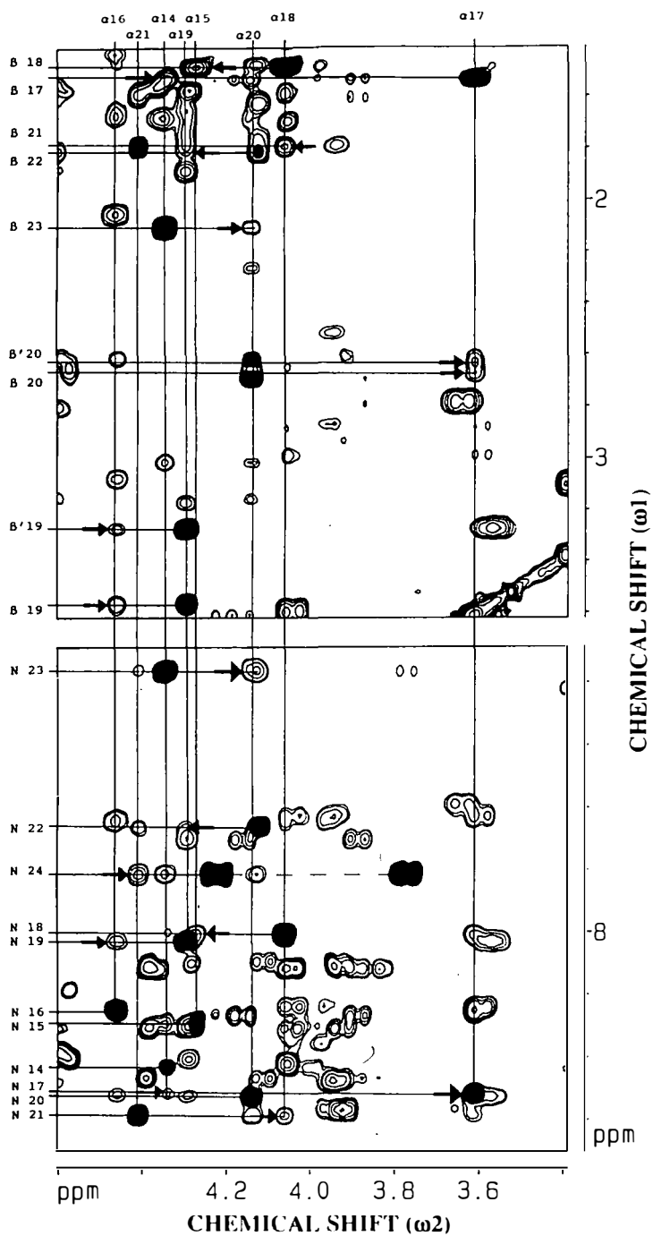
Fig. 5. Parts of a 500 MHz NOESY (150 ms) spectrum of recombinant defensin A in ^1\text{H}_2\text{O} (pH 4.9, 8.9 mM, 294 K). The \alpha\text{H} - \beta\text{H} and \alpha\text{H} -NH cross-peak regions covering residues from Ser 14 to Gly 24 are displayed at the top and bottom, respectively. NH, \alpha\text{H} and \beta\text{H} chemical shifts are enhanced by solid lines. A dashed line connects the two doublets of Gly 24 (bottom). Black filled cross peaks denote intraresidual NOEs from Ser 14 to Gly 24 and arrows indicate (i, i + 3) connectivities.
