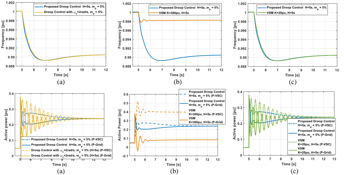
Figure 8: Comparison of the proposed method to conventional ones (a) Conventional droop control with H=5s, (b) VSM with high damping coefficient, (c) VSM with a small damping coefficient equivalent to the droop gain.
