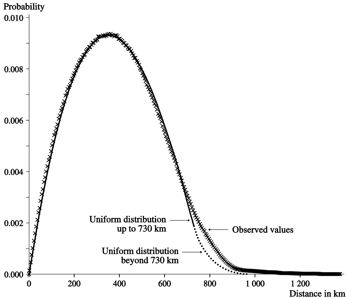
Figure 6. Sampled frequency distribution of distances (indicated by crosses “x”) between 1 \text{ km} \times 1 \text{ km} squares for France compared with the theoretical probability density function of distances between random pairs of points from a square with side 728 km (solid line up to 730 km, dotted line beyond).
