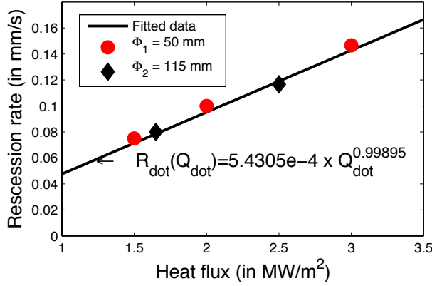
Figure 7: Recession rate in function of cold wall heat flux for the cork P50.
