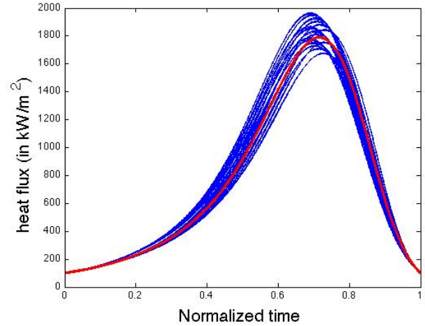
Figure 6: Heat flux profile with dispersion versus normalized time
