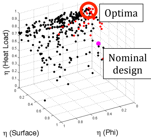
Figure 5: 3d plot representing the result of the optimisation with the nominal and the chosen optima
