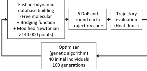
Figure 3: Methodology of the AeroSDS optimization
