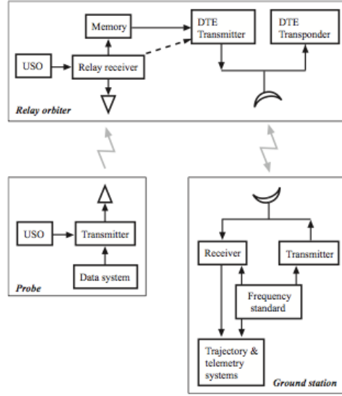
Figure 9: Relay communication system, from [8]
