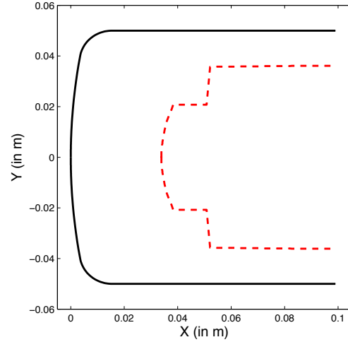
Figure 8: Cut of the heat shield (solid line: the external surface; dash line: inner surface)
