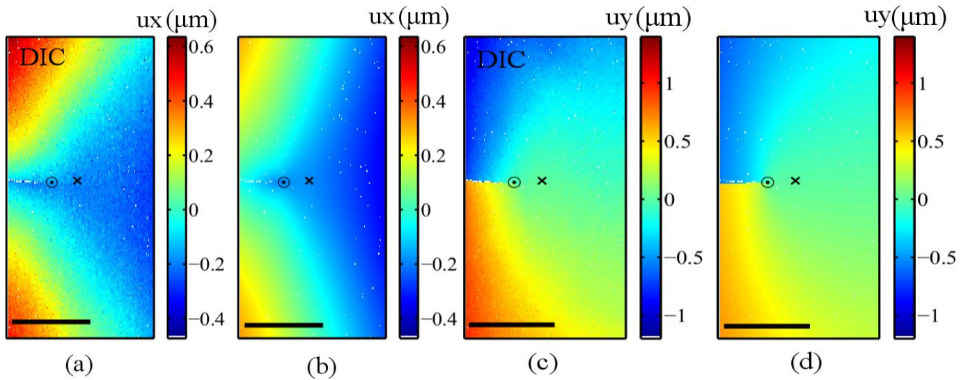
Fig. 9: Comparisons between the kinematic fields obtained by DIC (component u_x (a) and u_y (c)) and the optimized Williams' displacement fields (component u_x (b) and u_y (d)) for F = 620N
