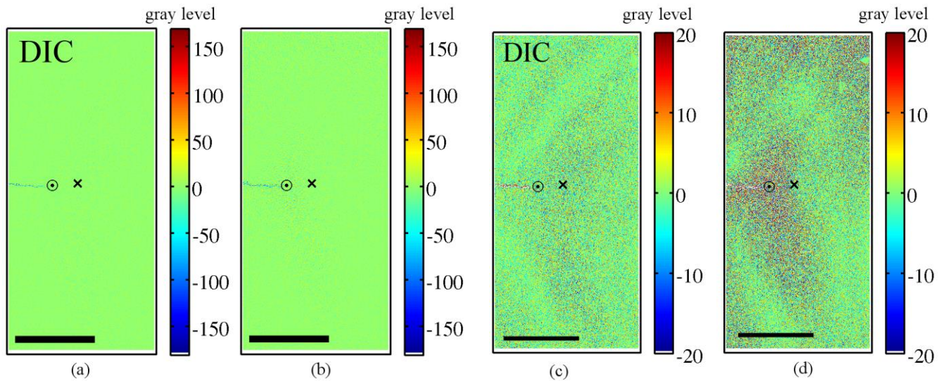
Fig. 10: Residual maps for the DIC ((a),(c)) and the Williams' expressions ((b),(d)) with a thresholded colorbar of values ((c),(d)) to highlight the low values of residuals ( F = 620N ). The colorbars correspond to gray levels coded in 8 bits
