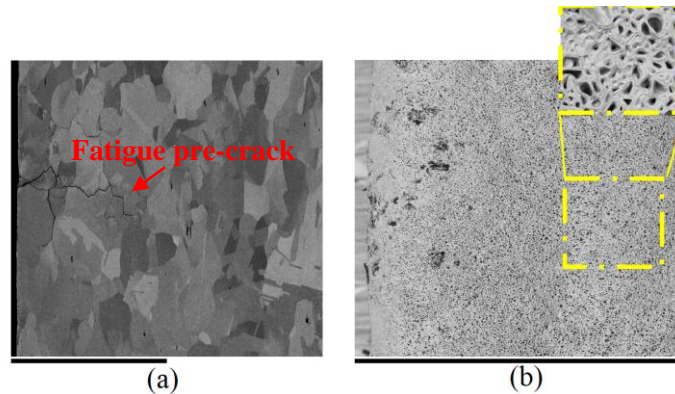
Fig. 2: Inter/trans-granular fatigue crack path appears at SENT surface after fine polishing (a) but cannot be monitored after preconditioning treatment (b). The scale bar is 500 µm and the square length is 35 µm
