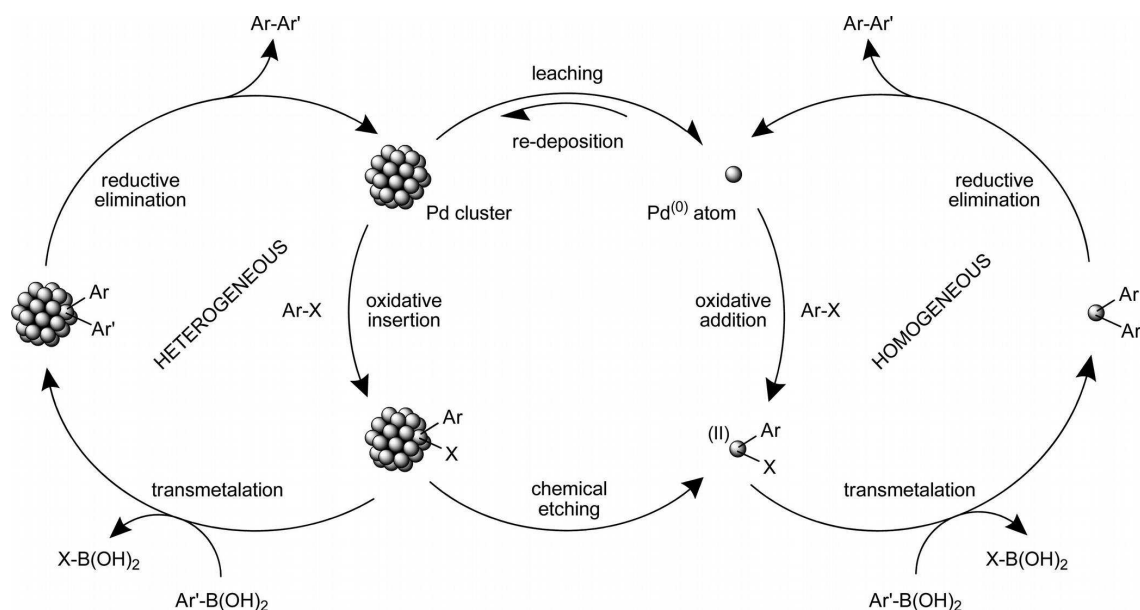
Figure 1. Proposed mechanism for the PdNP-catalyzed Suzuki cross-coupling involving both homogeneous and "heterogeneous" pathway, reprinted with permission from [14]. Copyright (2012) American Chemical Society. Please note that both act in the liquid phase.
