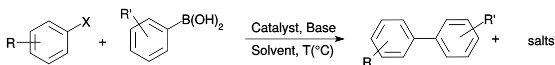
Figure 3. Schematic representation of the Suzuki coupling - R' = H (otherwise specified).
