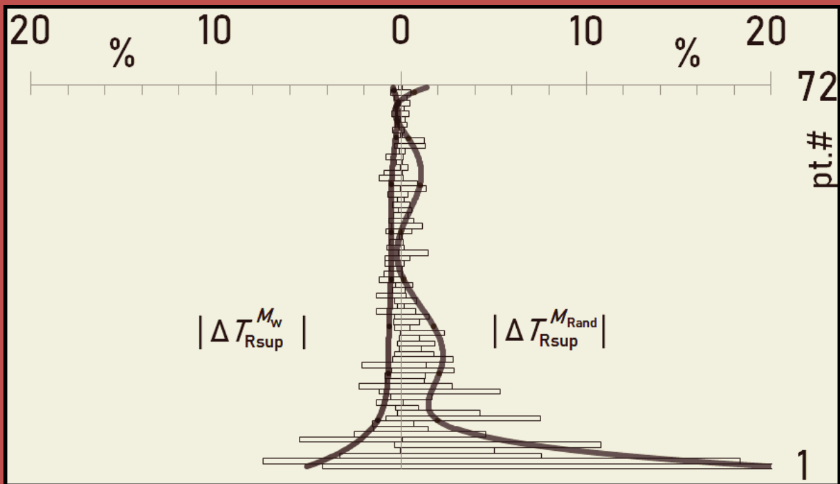
Absolute outperformance of real-data ( M_w seismic magnitudes) spectra over random-data spectra in matching the 72h period-forced superharmonic resonance's 72 theoretical subperiods. Polynomial trendlines overlaid.
