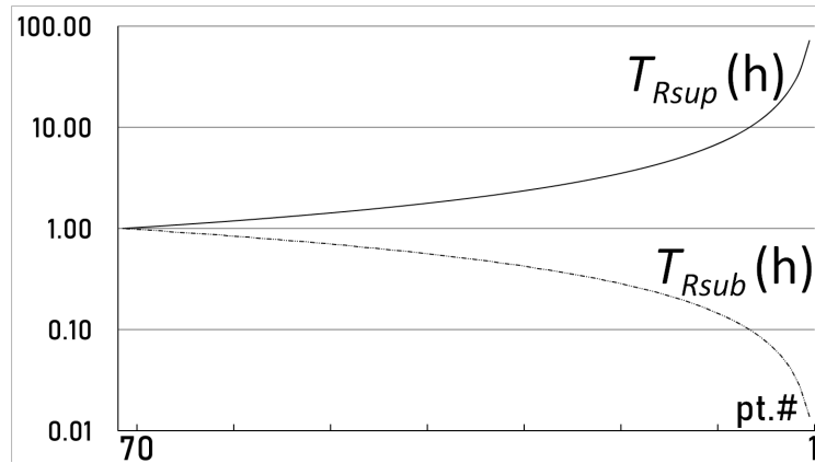
Figure 4. The full range (all 72) of the 3-day phase’s theoretical superharmonic-resonance periods: (72/72) h, (72/71) h, (72/70) h, ... (72/1) h, Figure 3, (solid line), v. the full range of the complementing theoretical subharmonic resonance periods: (72/72) h, (71/72) h, ... (1/72) h (dashed line). Abscissa values in reverse-order for legibility.
