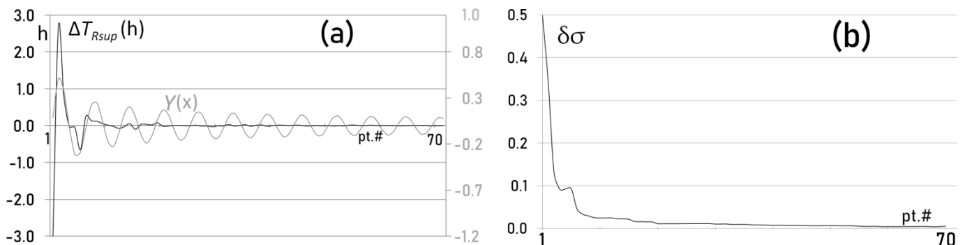
Figure 6. Difference \Delta T_{Rsup} in hours (dark line; panel a) between the theoretical v. computed resonance periods from the earthquake occurrence spectra that have revealed the Earth’s superharmonic resonance, Table 2 and Figure 3. At first sight, the difference seems best modeled by a mother half-wavelet function. But due to the fixed precision of spectral analyses to 10^{-4} or better than 4 s at 1Hz data sampling rate, as well as finiteness of the resonance range and discreteness of the resonating masses, the standard deviation divergence \delta\sigma , Table 2, at first changes considerably with lowering the number of differences taken into account, only to stabilize asymptotically rather quickly (panel b). So the difference could, in reality, reflect the overall system’s response to superharmonic resonance in the form of the Bessel equation (light line; panel a), specifically an asymptotically fast-converging Weber function Y(x) , Eqn. (14). Since the Weber function is a type of the Bessel (parabolic cylindrical) functions, this approximation reflects the clustering tendency of global seismicity towards low latitudes, as well as the origin of the North-South preferential orientation of tectonics.
