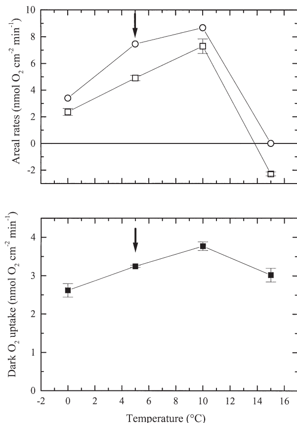
Fig. 3. Temperature effects on net productivity (□), gross photosynthesis (○) and dark O 2 uptake (■) in the artificial microbial mat. Areal rates were calculated from the data presented in Fig. 1. The arrows indicate the temperature originally used for culturing the mat. Error bars are \pm 1 SD ( n = 3 )
