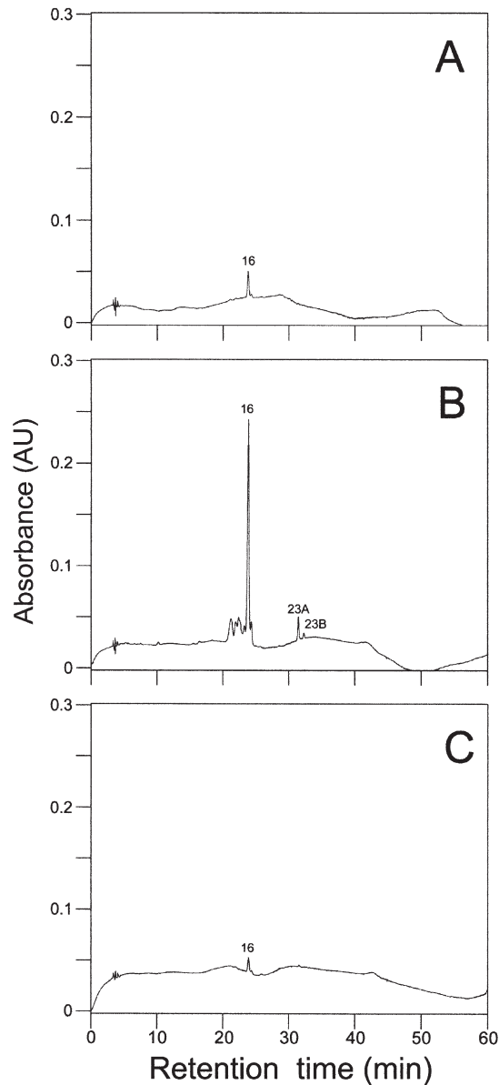
Fig. 2. Absorbance chromatograms at 770 nm of extracts of Artificial Mat 2 samples from (A) the upper green layer, (B) the underlying pink layer, and (C) the colourless sand underlying the mat. For peak identification see Table 1
