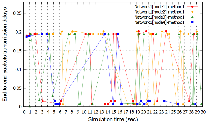
Figure 12 – End-to-end delays variations after resource allocation in network1 with method1.
