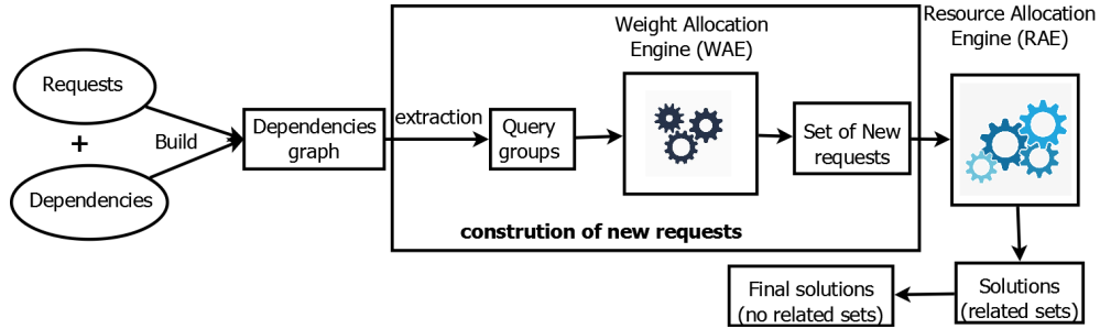
Figure 5 – Our resource allocation approach for interdependent requests.
