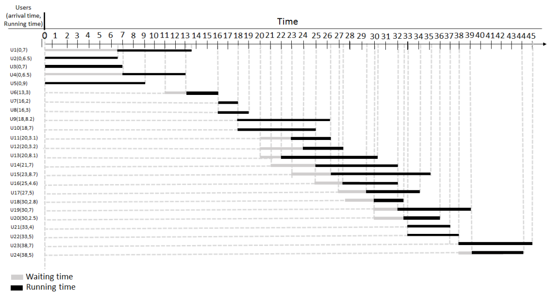
Figure 16 – Gantt chart for 24 sequential arrivals.
