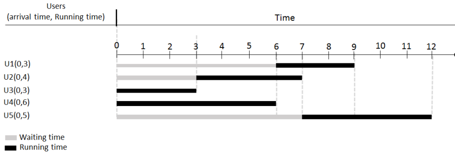
Figure 4 – Gantt chart for a set of five applicants for resources.
