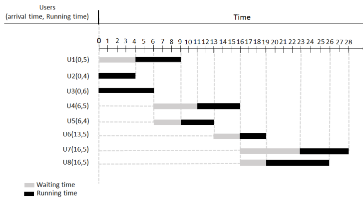
Figure 15 – Gantt chart for 8 sequential arrivals.
