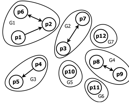
Figure 9 – New requests from the connected components of the graph.
