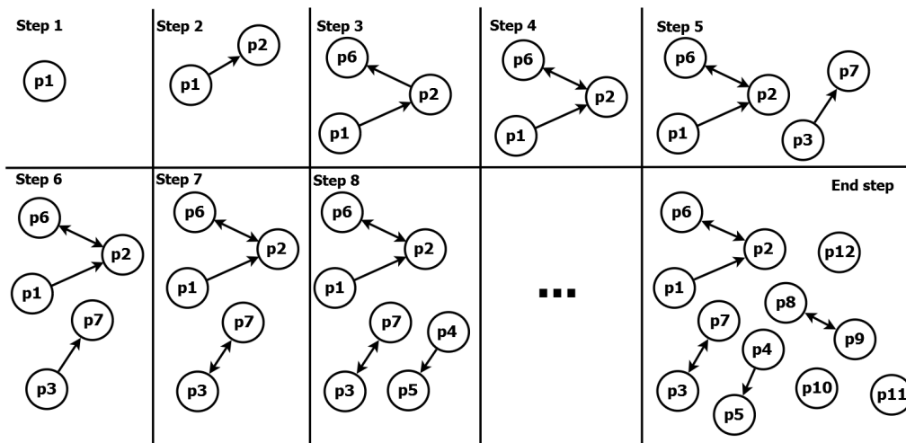
Figure 7 – Disconnected dependency graph construction process.
