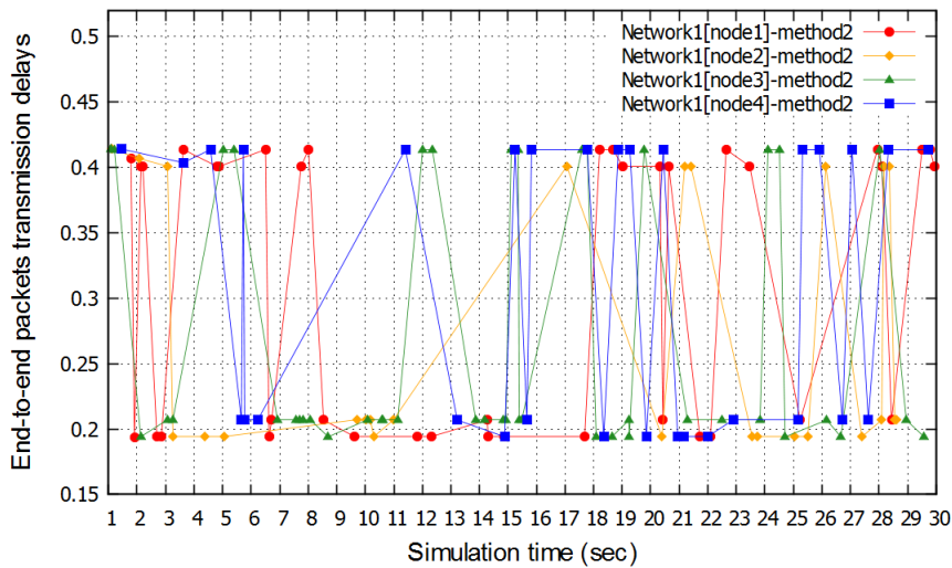
Figure 13 – End-to-end delays variations after resource allocation in network1 with method2.
