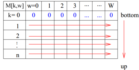
Figure 3 – Bottom-up computation principle.
