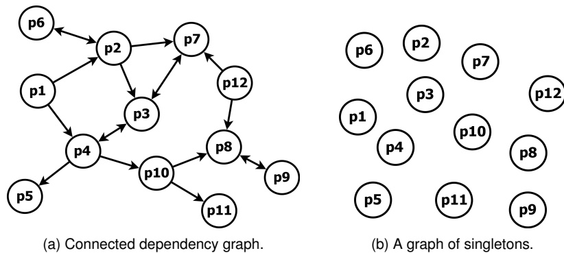
Figure 8 – Connected dependency graph and graph of singletons.
