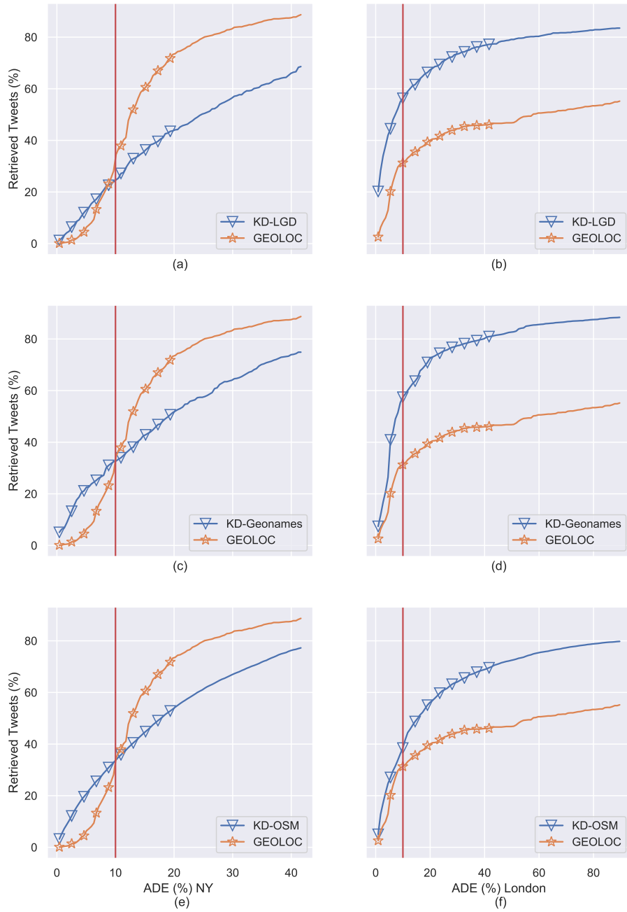
Fig. 1. ADE results using three semantic gazetteers.
