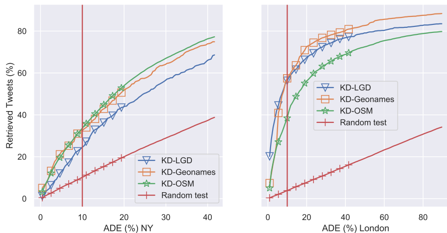
Fig. 2. Comparison among the three semantic gazetteers: results for NY (left), results for London (right).
