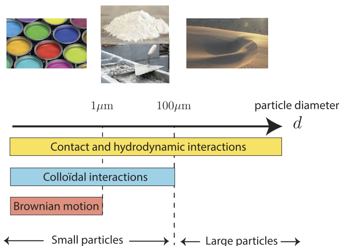
Fig. 1. Examples of granular media and illustration of the different interactions playing a role as a function of the size d of the particles.
