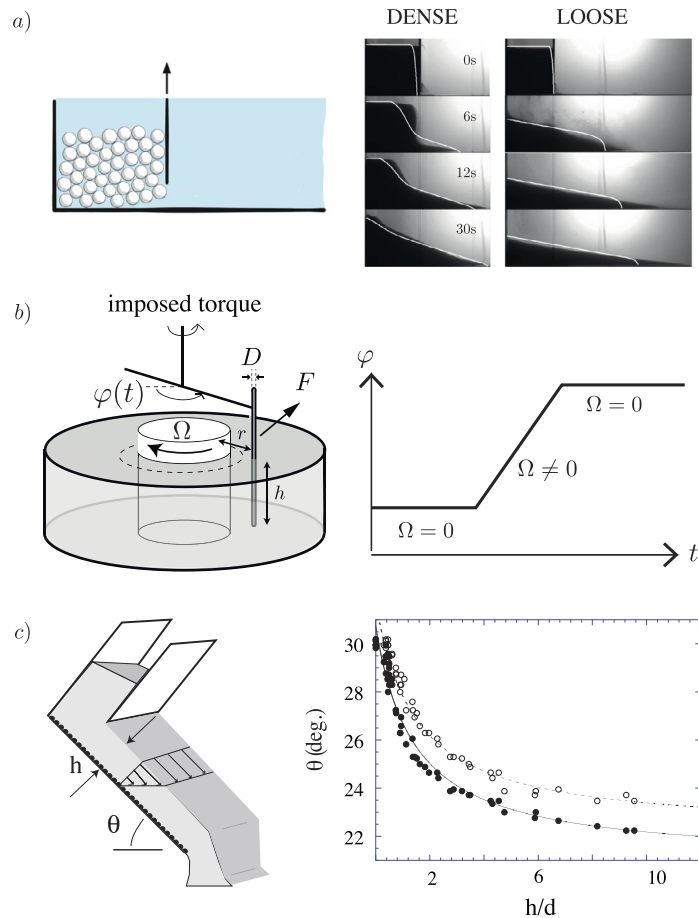
Fig. 5. a) Submarine collapse of granular column showing that the initial preparation of the packing in a dense or in a loose state strongly influences the dynamics [46]. b) Evidence of non-local effects in a Couette geometry: a rod submitted to a force F and immersed in the medium far from the shear band starts moving as soon as the inner cylinder rotates, although no macroscopic motion is observed around it [52]. c) Starting (open circles) and stopping (black dots) angles of a layer of grains on an inclined plane as a function of the thickness h/d of the layer [53].
