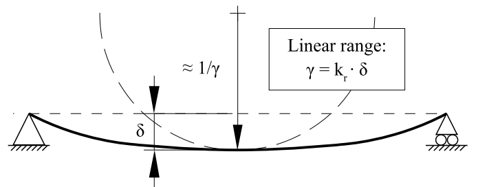
Figure 14: Displacement and curvature as engineering demand parameters
