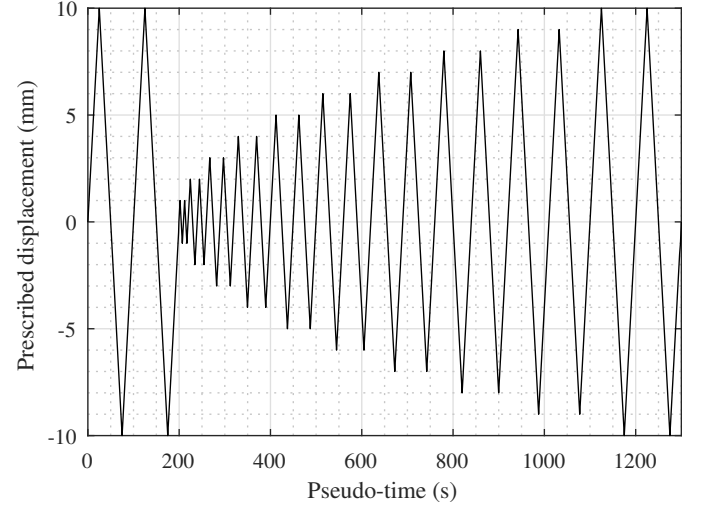
Figure 16: Loading procedure for the sensitivity study (example for \Gamma = 0.091 )
