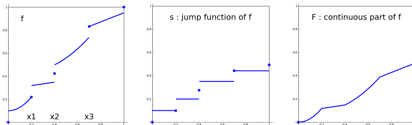
Figure 3: The fraphs of f , its jump function s and F = f - s .
