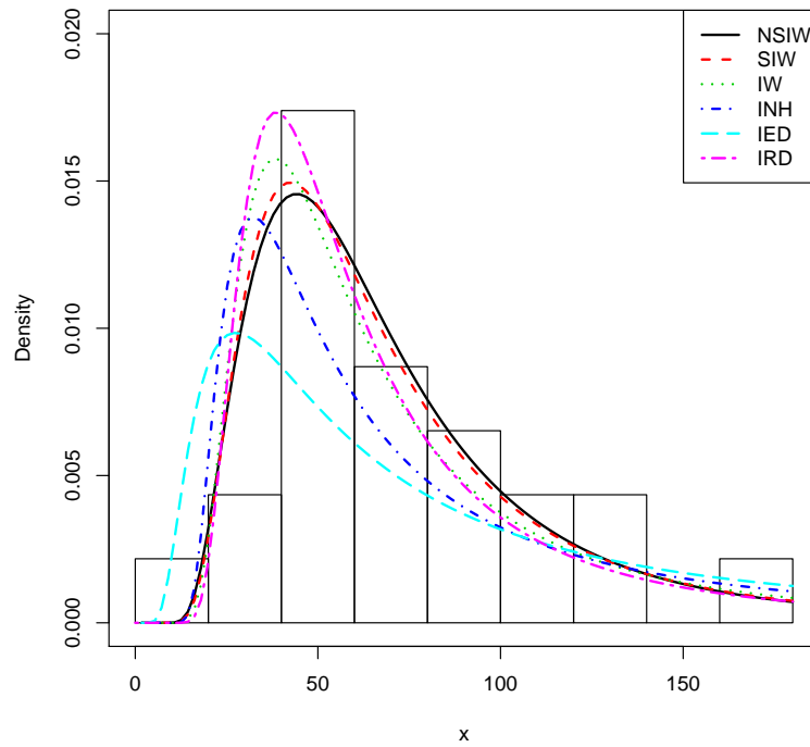
Figure 7: Plots of the estimated pdfs for data set 2.
