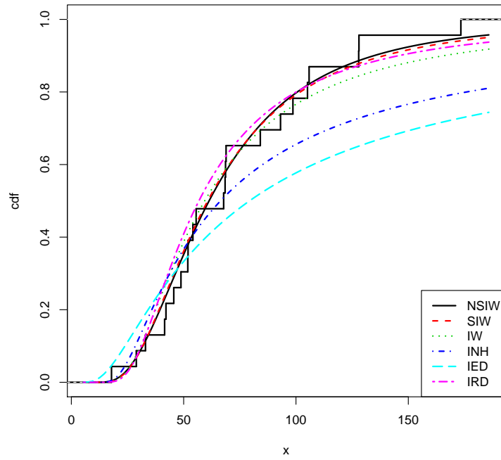
Figure 9: Plots of the estimated cdfs for data set 2.
