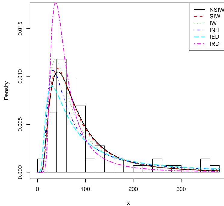
Figure 6: Plots of the estimated pdfs for data set 1.
