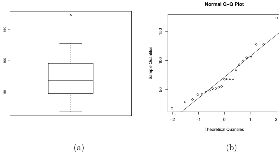
Figure 5: (a) Boxplot (b) Normal Q-Q plot for data set 2.
