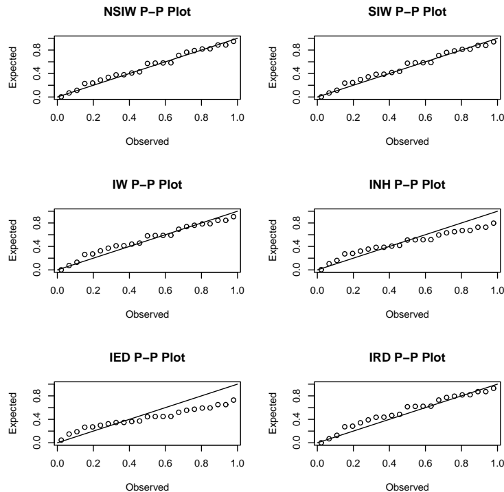
Figure 11: P-P Plots of the estimated models for data set 2.
