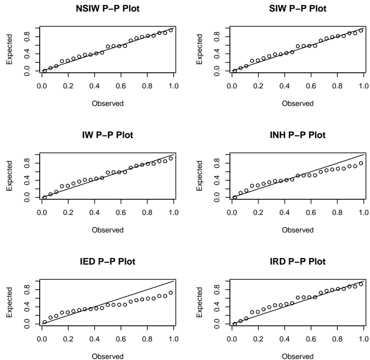
Figure 11: P-P Plots of the estimated models for data set 2.
