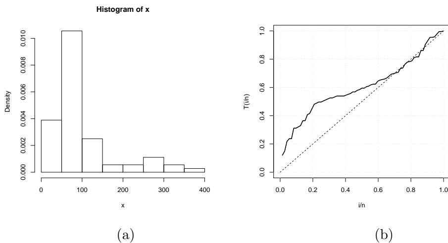
Figure 2: (a) Histogram (b) TTT plot for data set 1.
