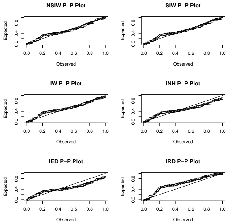
Figure 10: P-P Plots of the estimated models for data set 1.
