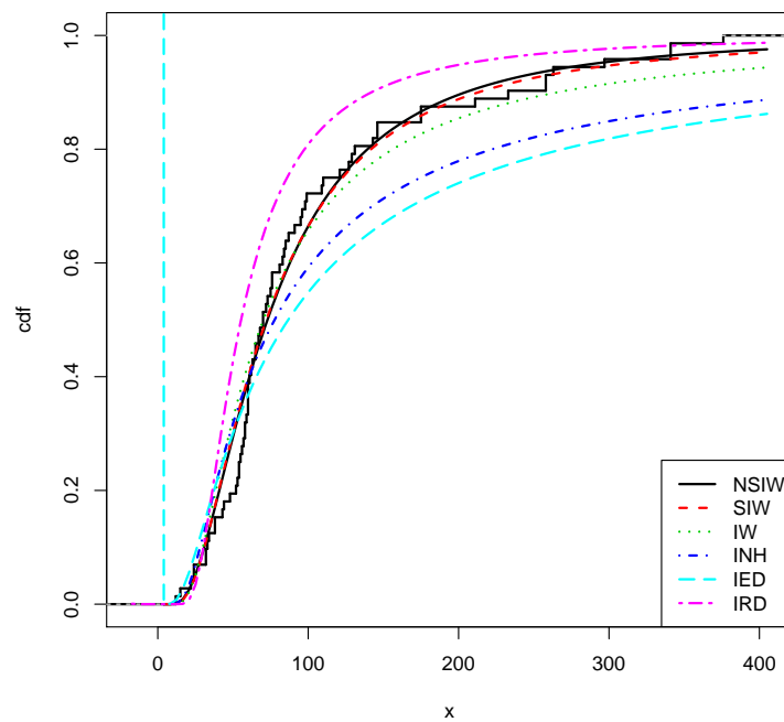
Figure 8: Plots of the estimated cdfs for data set 1.
