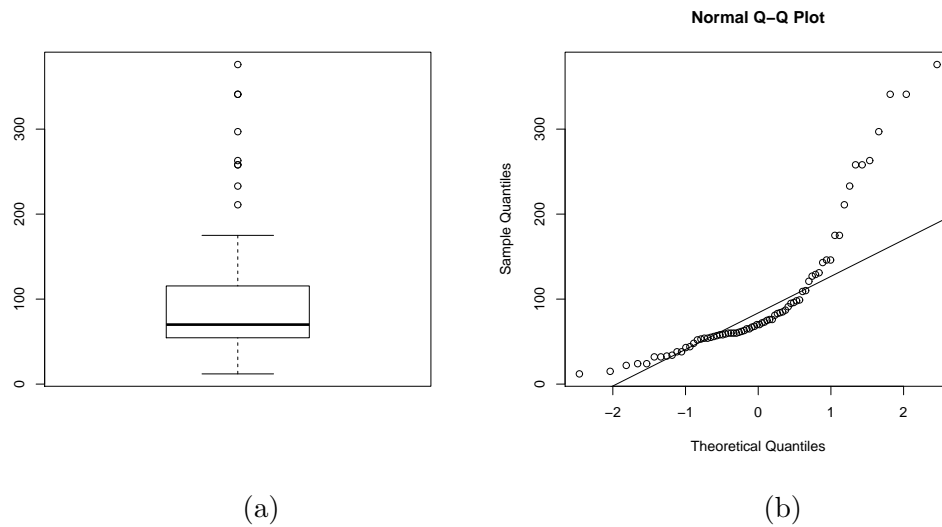
Figure 3: (a) Boxplot (b) Normal Q-Q plot for data set 1.
