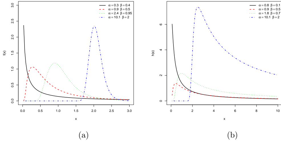
Figure 1: (a) Curves for the pdf f(x) (b) Curves for the hrf h(x) for selected values of the parameters.
