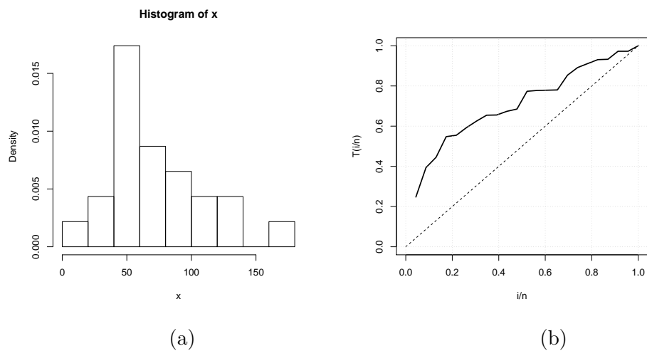
Figure 4: (a) Histogram (b) TTT plot for data set 2.
