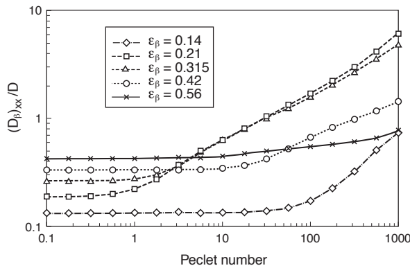
Figure 5 Transversal dispersion coefficient versus the unit cell Peclet number and for various saturations.
