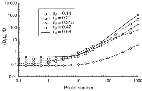
Figure 4 Longitudinal dispersion coefficient versus the unit cell Peclet number and for various saturations.
