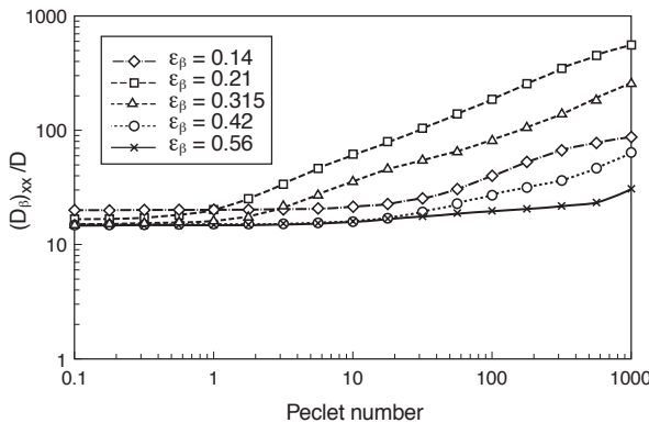
Figure 6 Mass exchange coefficient versus the unit cell Peclet number and for various saturations.
