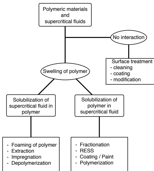
Figure 11 Schematic CO 2 -polymer interactions and potential applications.
