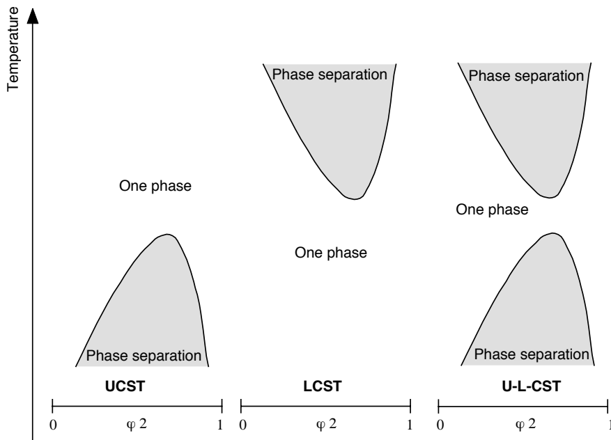
Figure 14 Binodal curves in systems displaying UCST, LCST and U-L-CST.
