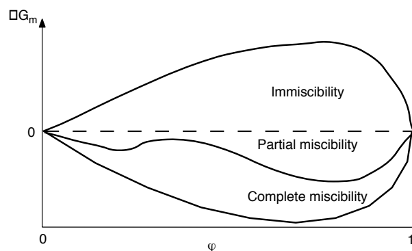
Figure 12 Schematic Gibbs free energy of a mixture with respect to the polymer concentration.
