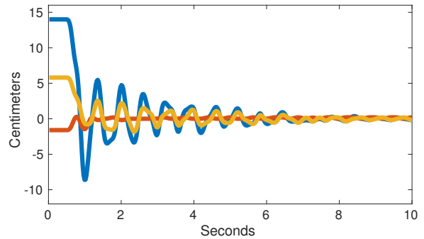
Fig. 4. Open-loop arm experiment starting from an actuated and deformed state going towards a straight, down-hanging arm pose. The graph shows the x (red), y (blue) and z (yellow) positions of the arm's end-effector as it is swinging back and fourth while asymptotically nearing a straight arm pose.
