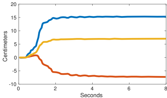
Fig. 8. Simulation of closed-loop control, showing the motion of the end-effector going from the straight resting pose to an actuated state. Red, blue and yellow lines show position along x, y and z axis.
