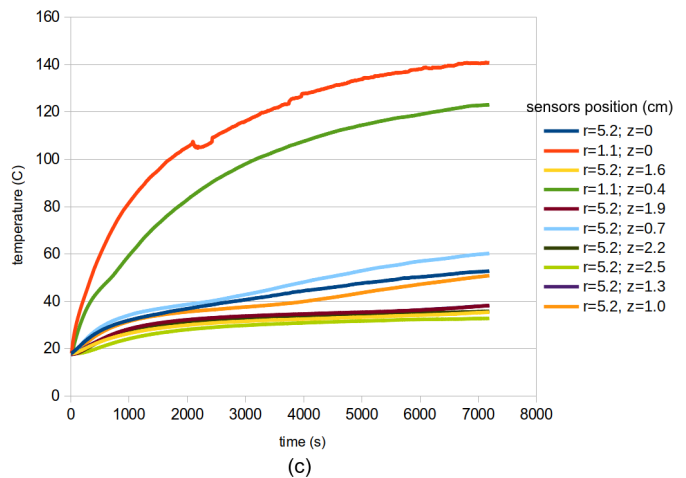
Figure 3: (a) Sketch of the laboratory heating device. The multiple reflections of the IR rays inside the aluminum cylinder produces a uniform heat flux at the surface of the sand. The sand box and the heating are both axisymmetric. On right: Laboratory Experiment #1 (LE#1, above) and #2 (LE#2, below). Temperature versus time, at different position (cm) in the sample. Dry sand (b) or humid sand (c) with saturation S=8\% , heated by a constant flux infrared device. Curves are typically smooth in case (b), but may present an inflection point (c), related to the evaporation of a low water content in the sample.
