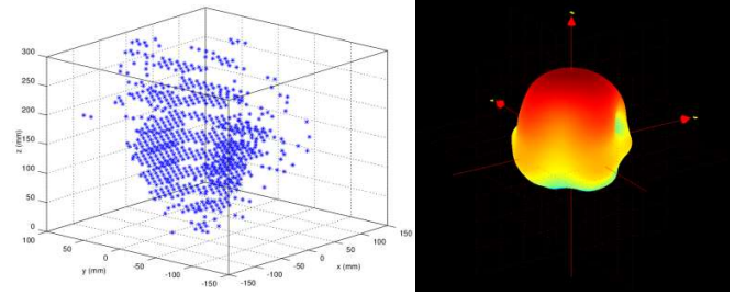
Fig. 3. 3D characterization: (a) Representation of the volume in which the tag is correctly read; (b) Radiation pattern measured for vertical horn of the antenna, at 5.5 GHz.
