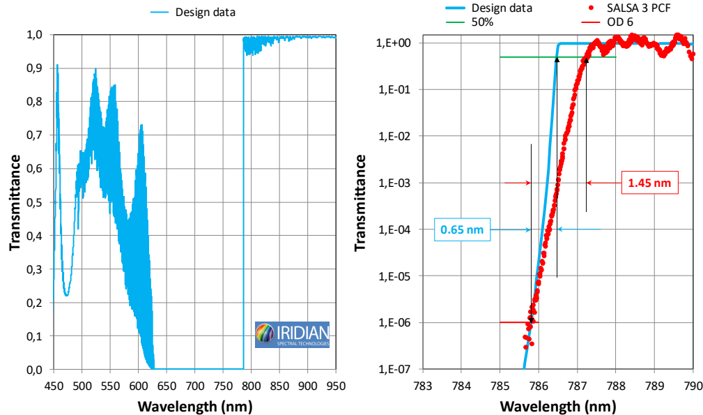
Fig. 9. Characterization of the steepness of a band edge filter manufactured by IRIAN Spectral Technologies (NanoEdge 785).
