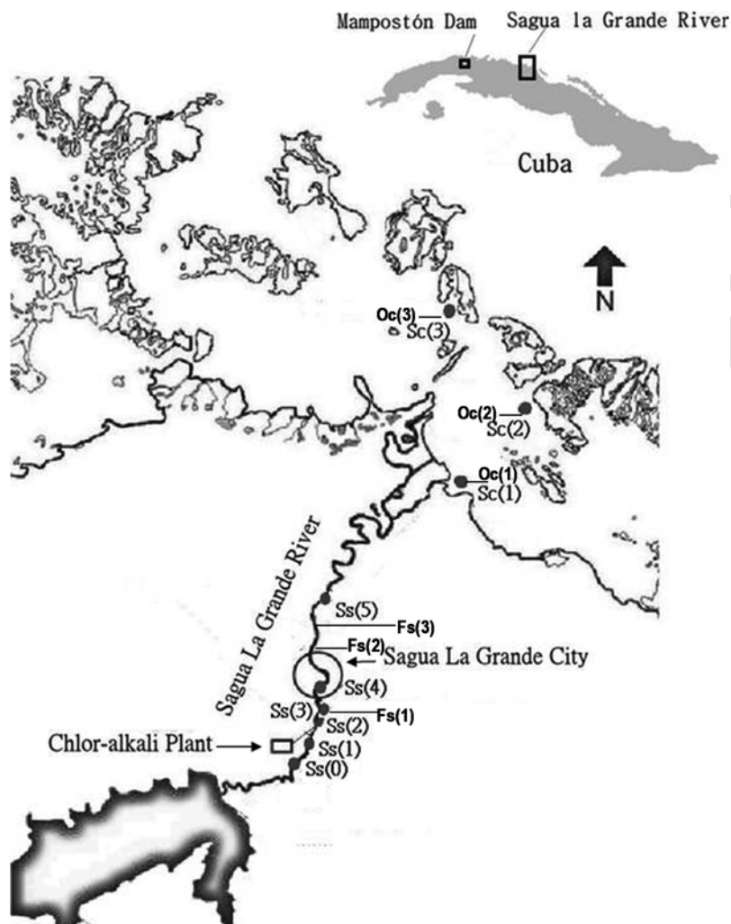
Fig. 1. Study area: Sagua la Grande River (SG River) and the adjacent (12 km) coastal zone (Cuba). Sediments sampling sites Ss(0) to Ss(5) are within the SG River, including Ss(1) in the vicinity of old CAP discharge, and Ss(2) and Ss(3) that are close to the new CAP discharge. Sc(1) to Sc(3) are in the coastal zone. Fish samples were collected in SG River, oyster samples were collected in coastal zone.
