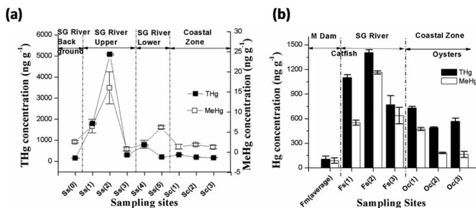
Fig. 2. Hg distribution and speciation in a) sediments and b) biota along SG River, coastal zone and M Dam.
