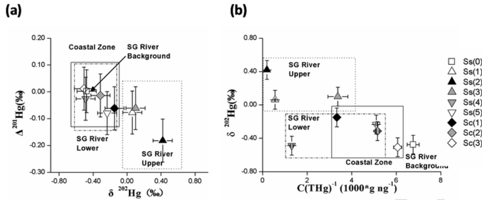
Fig. 3. a) \delta^{202}\text{Hg} relative to \Delta^{201}\text{Hg} isotopic composition and b) \delta^{202}\text{Hg} isotopic composition versus total Hg concentration in sediments of SG River and coastal zone.
