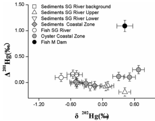
Fig. 4. \delta^{202}\text{Hg} and \Delta^{201}\text{Hg} isotopic composition in sediments and biota from SG River and coastal zone.
