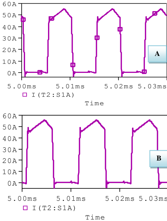
Figure .12 Output transformer current generated
