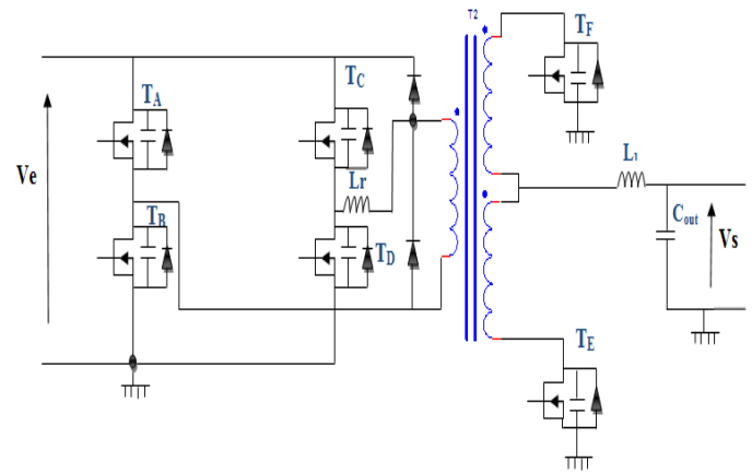
Figure1. DC/DC Full Bridge converter scheme
