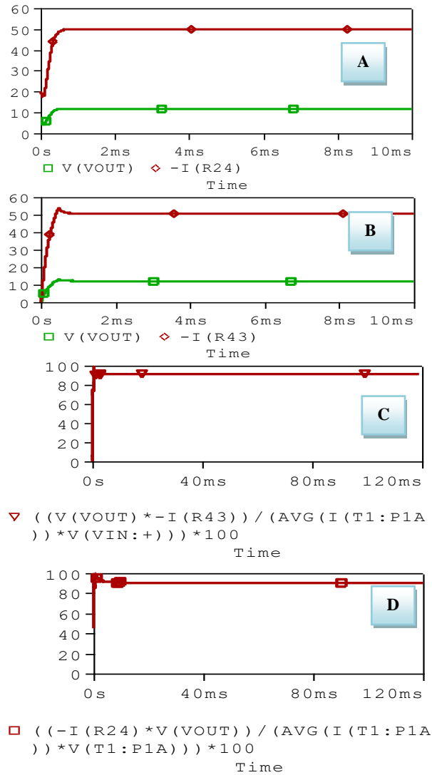
Figure. 13 Electrical quantities at the output of the DC/DC converter generated by the two controls:
